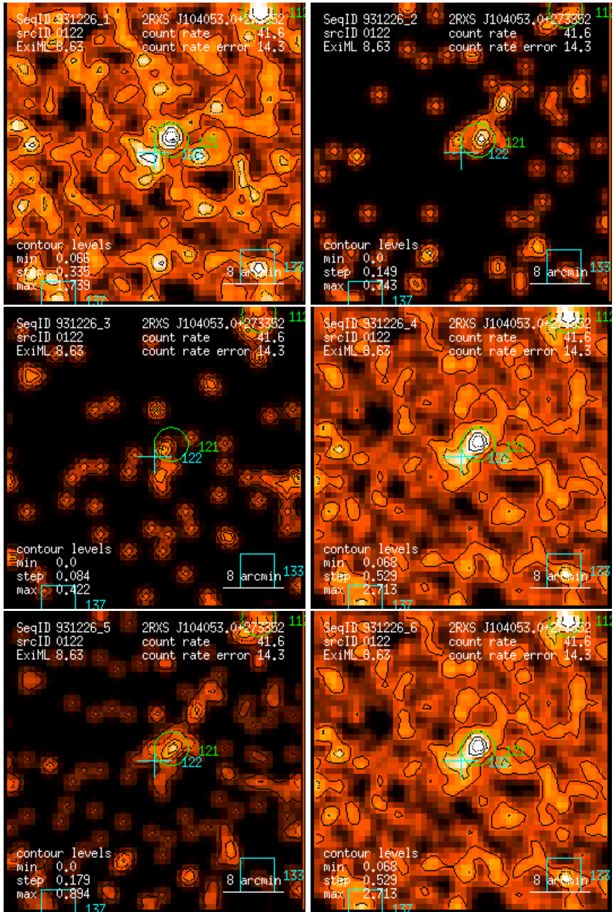
Figure 122: RASS 931226: detection 0122: band rate images, Gaussian filter: (1) PSPC channels 11 – 41, (2) 52 – 90, (3) 91 – 201, (4) 11 – 235, (5) 52 – 201, (6) 11 – 201. Broad band rates in counts/ks. Band rate contour levels in counts/ks/arcmin 2 .
