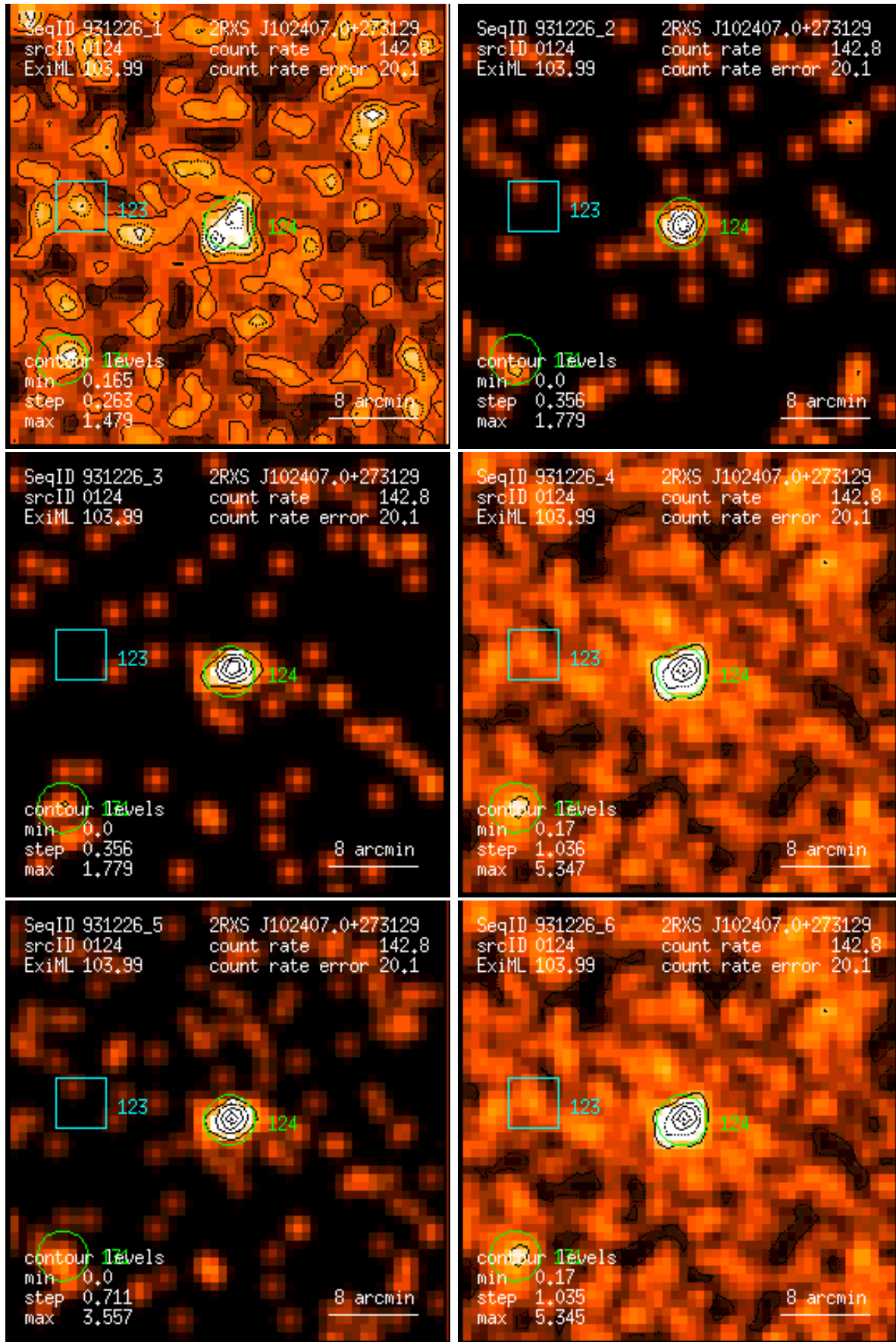
Figure 124: RASS 931226: detection 0124: band rate images, Gaussian filter: (1) PSPC channels 11 – 41, (2) 52 – 90, (3) 91 – 201, (4) 11 – 235, (5) 52 – 201, (6) 11 – 201. Broad band rates in counts/ks. Band rate contour levels in counts/ks/arcmin 2 .
