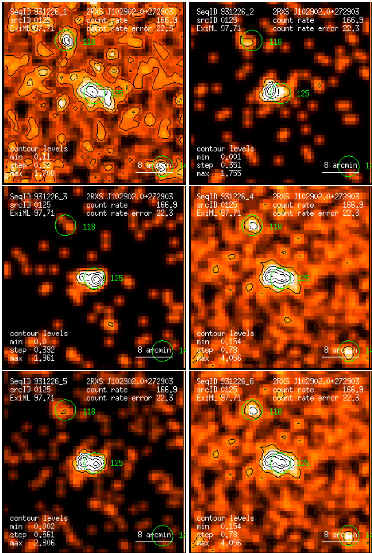
Figure 125: RASS 931226: detection 0125: band rate images, Gaussian filter: (1) PSPC channels 11 – 41, (2) 52 – 90, (3) 91 – 201, (4) 11 – 235, (5) 52 – 201, (6) 11 – 201. Broad band rates in counts/ks. Band rate contour levels in counts/ks/arcmin 2 .
