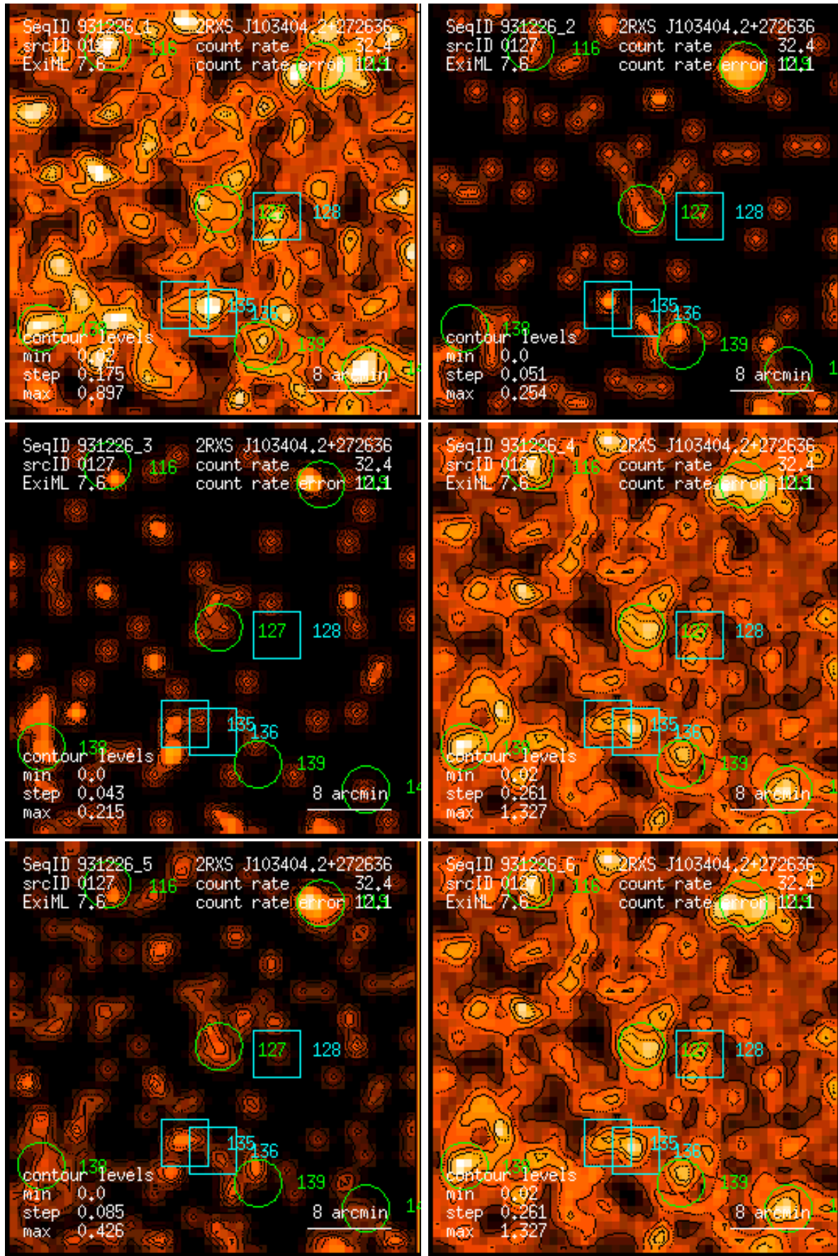
Figure 127: RASS 931226: detection 0127: band rate images, Gaussian filter: (1) PSPC channels 11 – 41, (2) 52 – 90, (3) 91 – 201, (4) 11 – 235, (5) 52 – 201, (6) 11 – 201. Broad band rates in counts/ks. Band rate contour levels in counts/ks/arcmin 2 .
