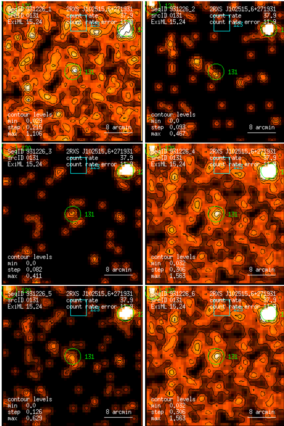
Figure 131: RASS 931226: detection 0131: band rate images, Gaussian filter: (1) PSPC channels 11 – 41, (2) 52 – 90, (3) 91 – 201, (4) 11 – 235, (5) 52 – 201, (6) 11 – 201. Broad band rates in counts/ks. Band rate contour levels in counts/ks/arcmin 2 .
