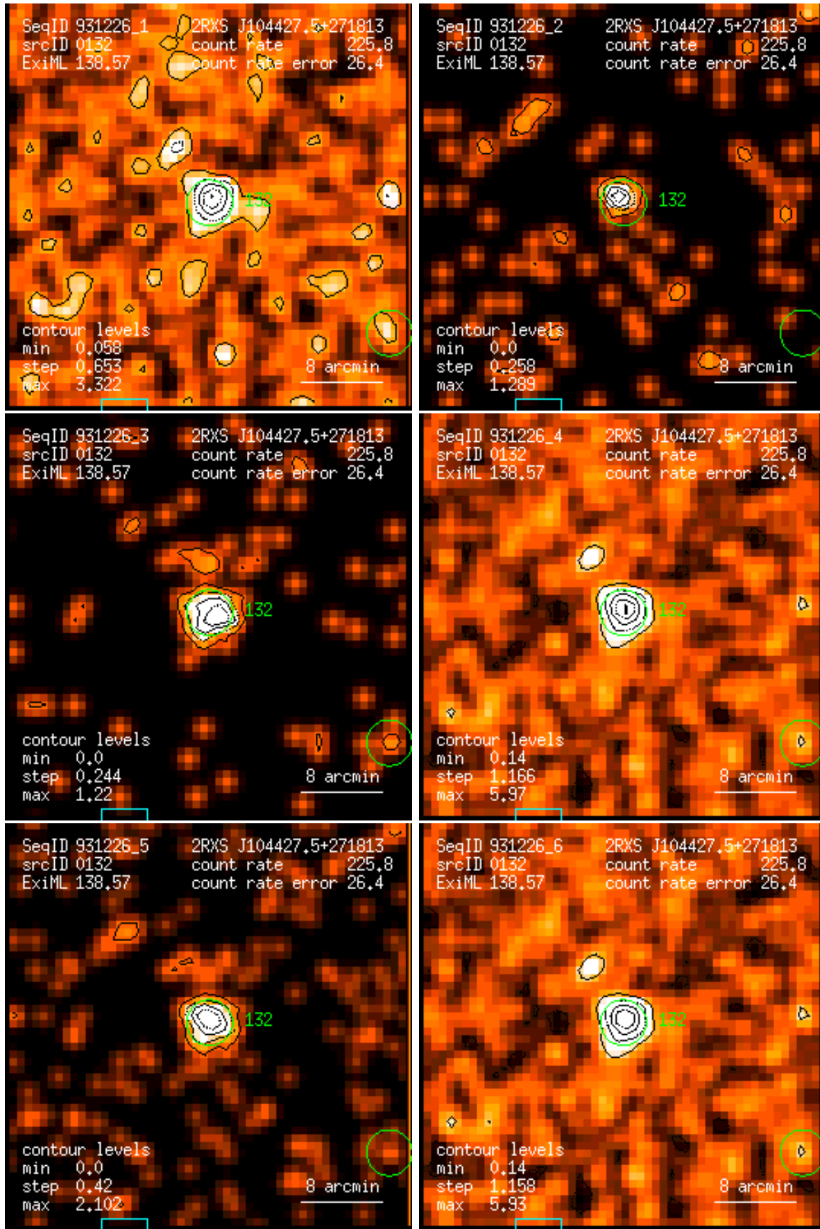
Figure 132: RASS 931226: detection 0132: band rate images, Gaussian filter: (1) PSPC channels 11 – 41, (2) 52 – 90, (3) 91 – 201, (4) 11 – 235, (5) 52 – 201, (6) 11 – 201. Broad band rates in counts/ks. Band rate contour levels in counts/ks/arcmin 2 .
