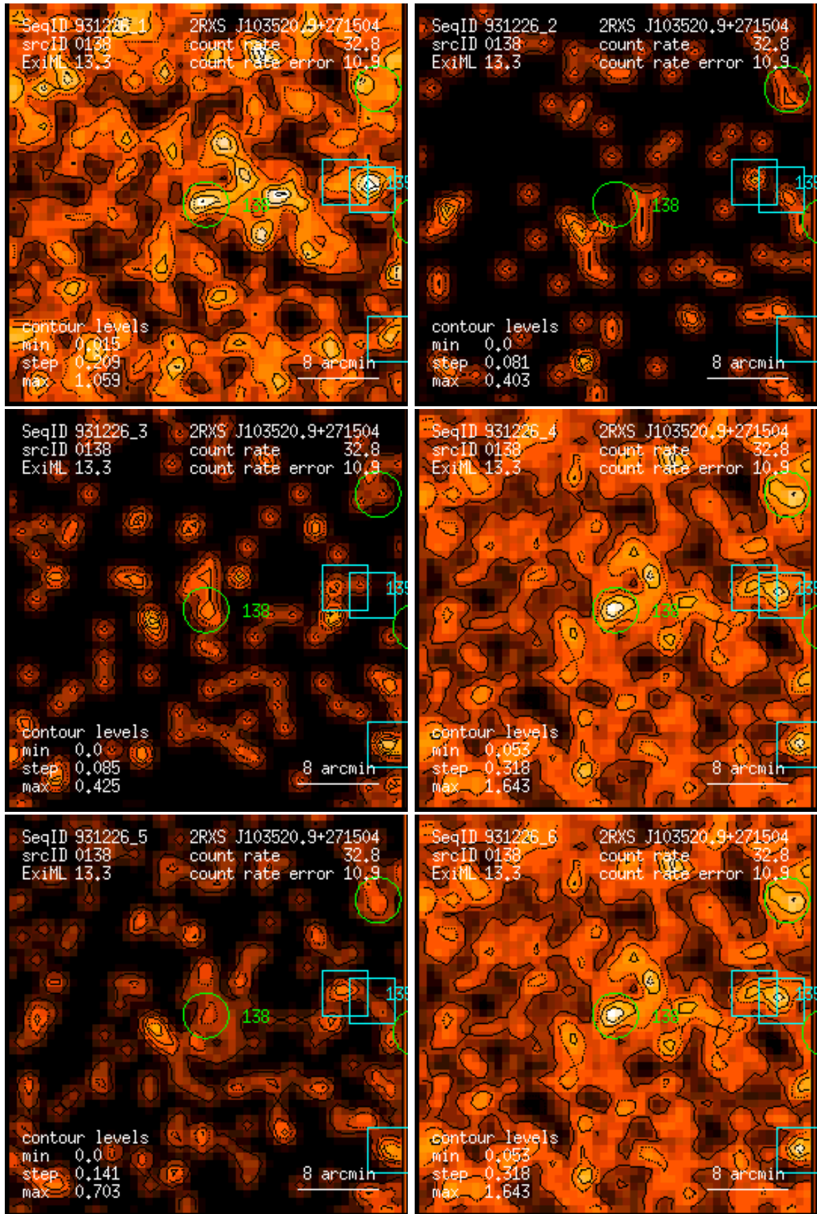
Figure 138: RASS 931226: detection 0138: band rate images, Gaussian filter: (1) PSPC channels 11 – 41, (2) 52 – 90, (3) 91 – 201, (4) 11 – 235, (5) 52 – 201, (6) 11 – 201. Broad band rates in counts/ks. Band rate contour levels in counts/ks/arcmin 2 .
