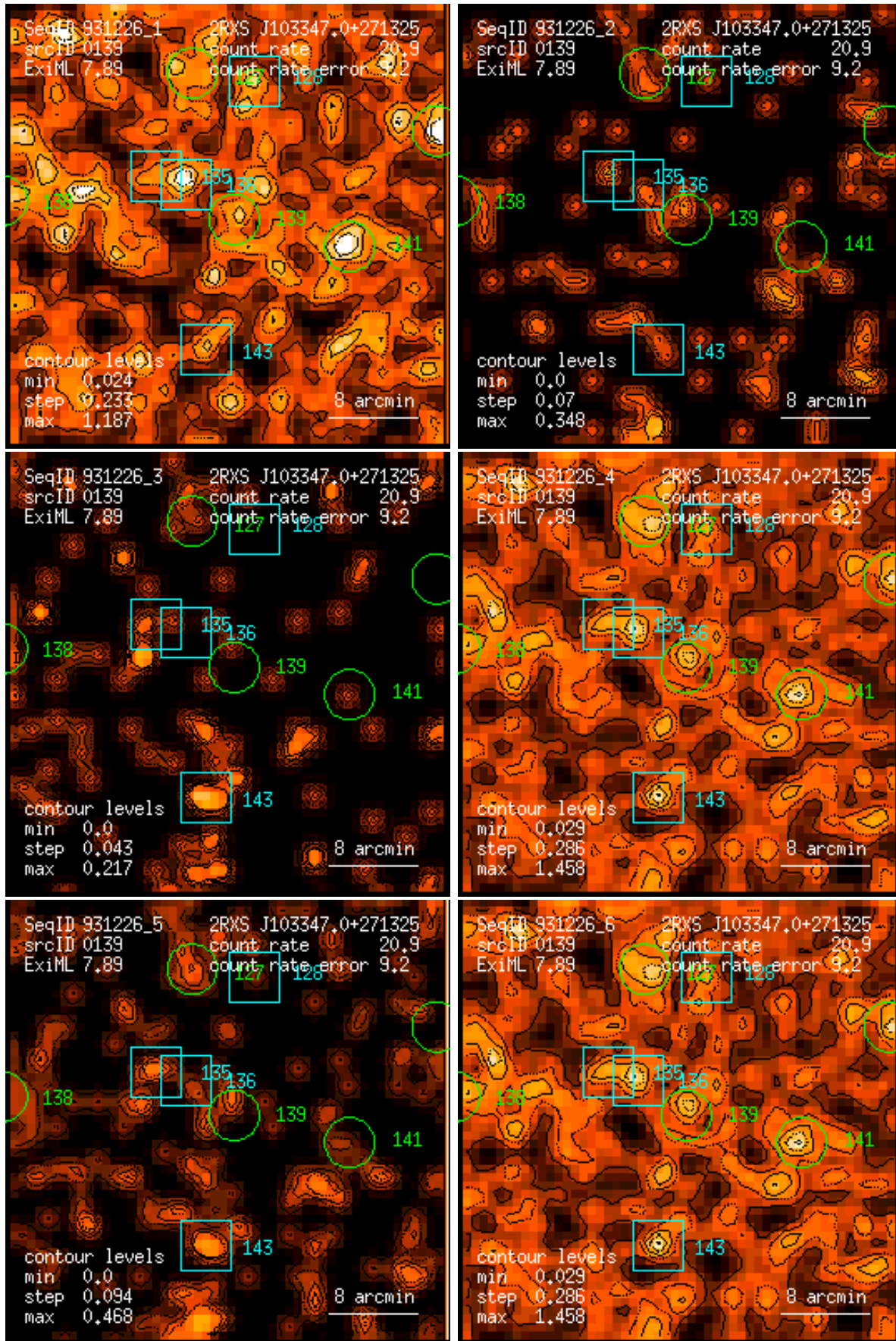
Figure 139: RASS 931226: detection 0139: band rate images, Gaussian filter: (1) PSPC channels 11 – 41, (2) 52 – 90, (3) 91 – 201, (4) 11 – 235, (5) 52 – 201, (6) 11 – 201. Broad band rates in counts/ks. Band rate contour levels in counts/ks/arcmin 2 .
