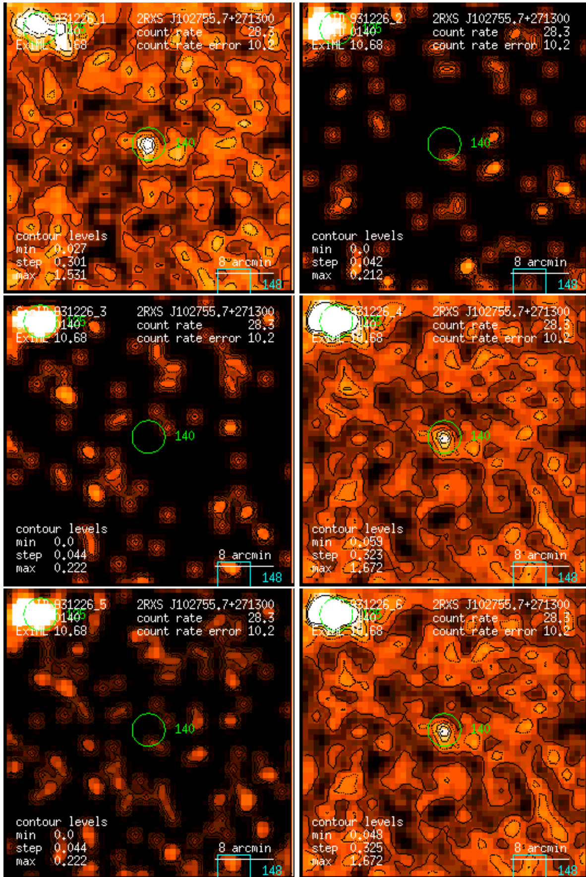
Figure 140: RASS 931226: detection 0140: band rate images, Gaussian filter: (1) PSPC channels 11 – 41, (2) 52 – 90, (3) 91 – 201, (4) 11 – 235, (5) 52 – 201, (6) 11 – 201. Broad band rates in counts/ks. Band rate contour levels in counts/ks/arcmin 2 .
