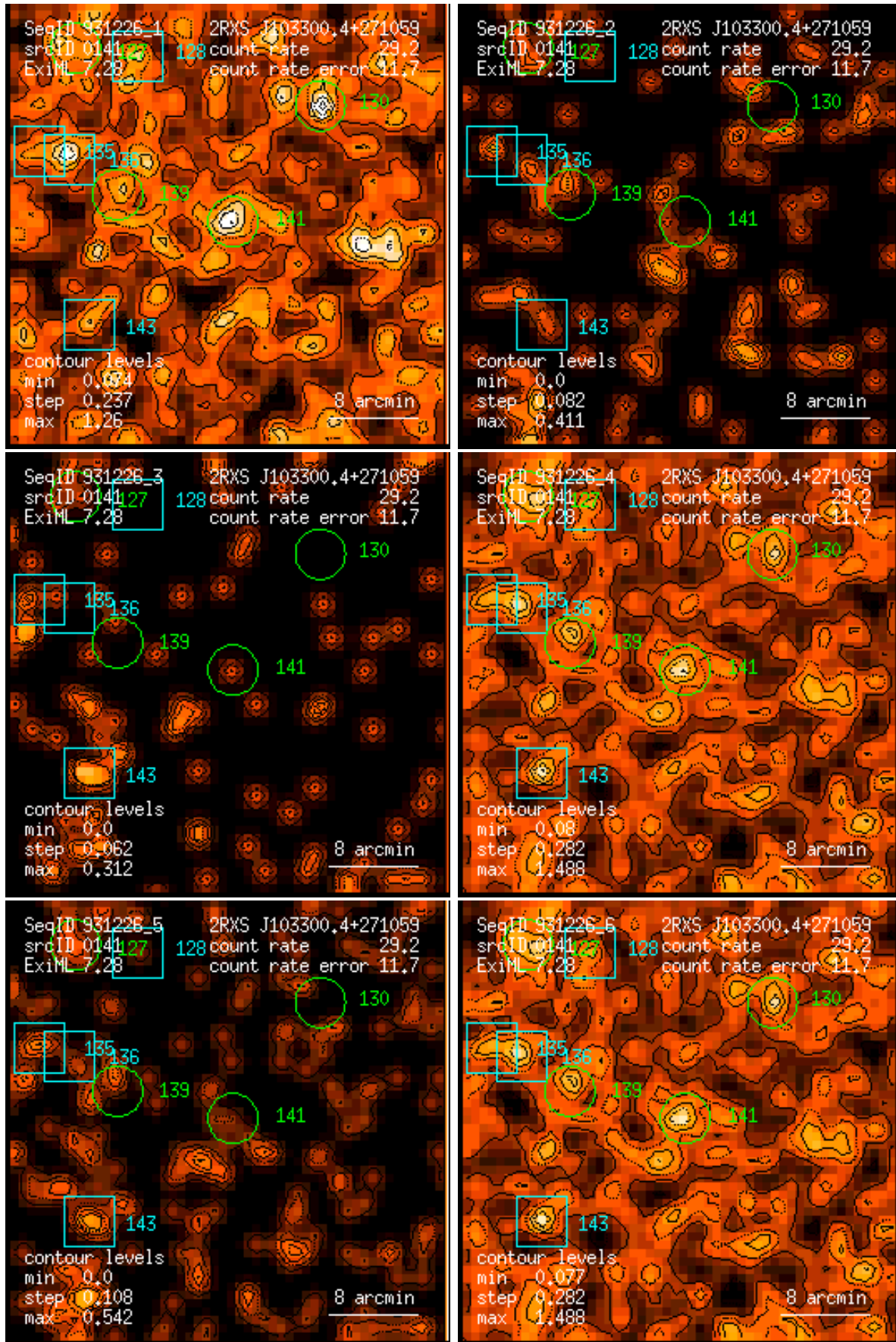
Figure 141: RASS 931226: detection 0141: band rate images, Gaussian filter: (1) PSPC channels 11 – 41, (2) 52 – 90, (3) 91 – 201, (4) 11 – 235, (5) 52 – 201, (6) 11 – 201. Broad band rates in counts/ks. Band rate contour levels in counts/ks/arcmin 2 .
