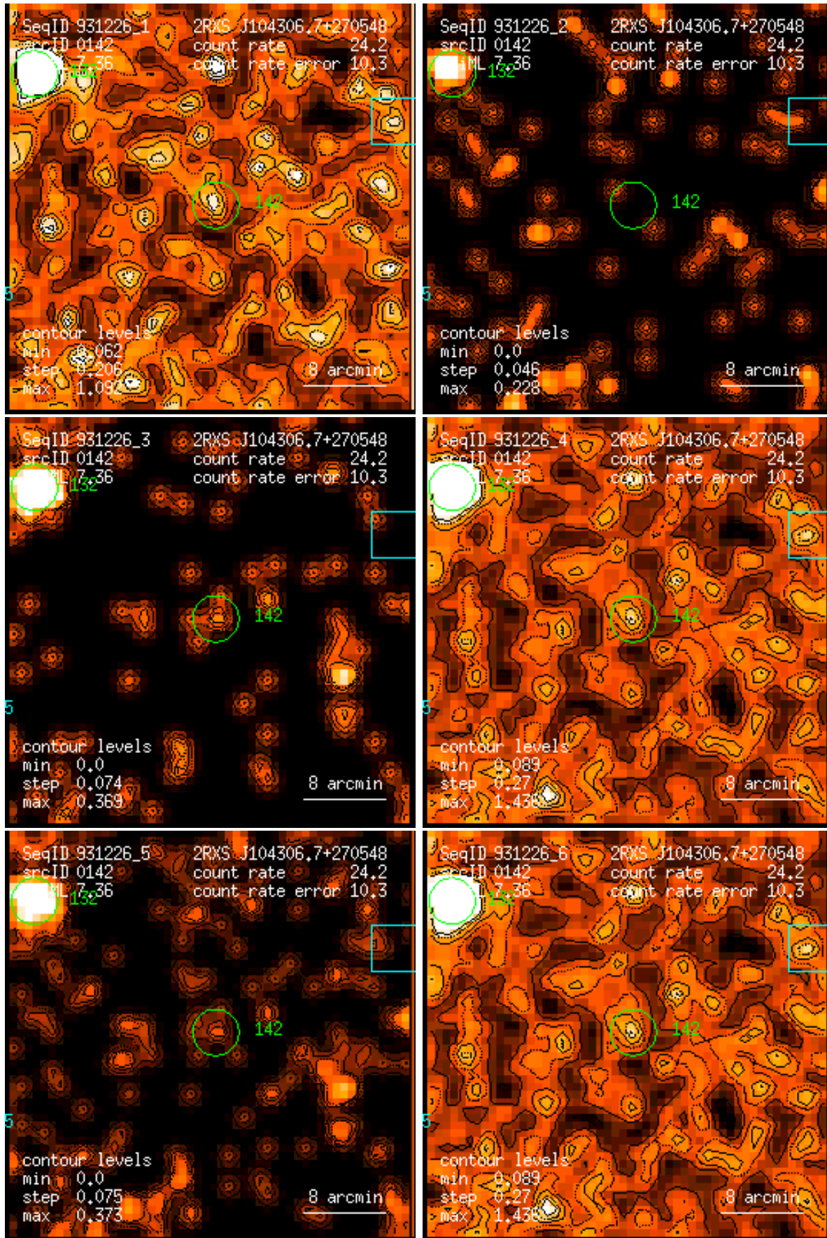
Figure 142: RASS 931226: detection 0142: band rate images, Gaussian filter: (1) PSPC channels 11 – 41, (2) 52 – 90, (3) 91 – 201, (4) 11 – 235, (5) 52 – 201, (6) 11 – 201. Broad band rates in counts/ks. Band rate contour levels in counts/ks/arcmin 2 .
