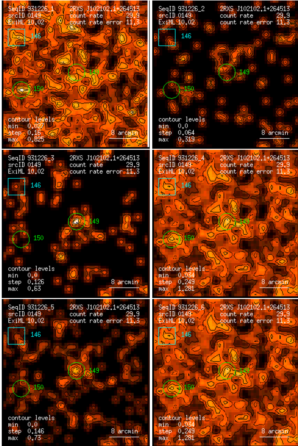
Figure 149: RASS 931226: detection 0149: band rate images, Gaussian filter: (1) PSPC channels 11 – 41, (2) 52 – 90, (3) 91 – 201, (4) 11 – 235, (5) 52 – 201, (6) 11 – 201. Broad band rates in counts/ks. Band rate contour levels in counts/ks/arcmin 2 .
