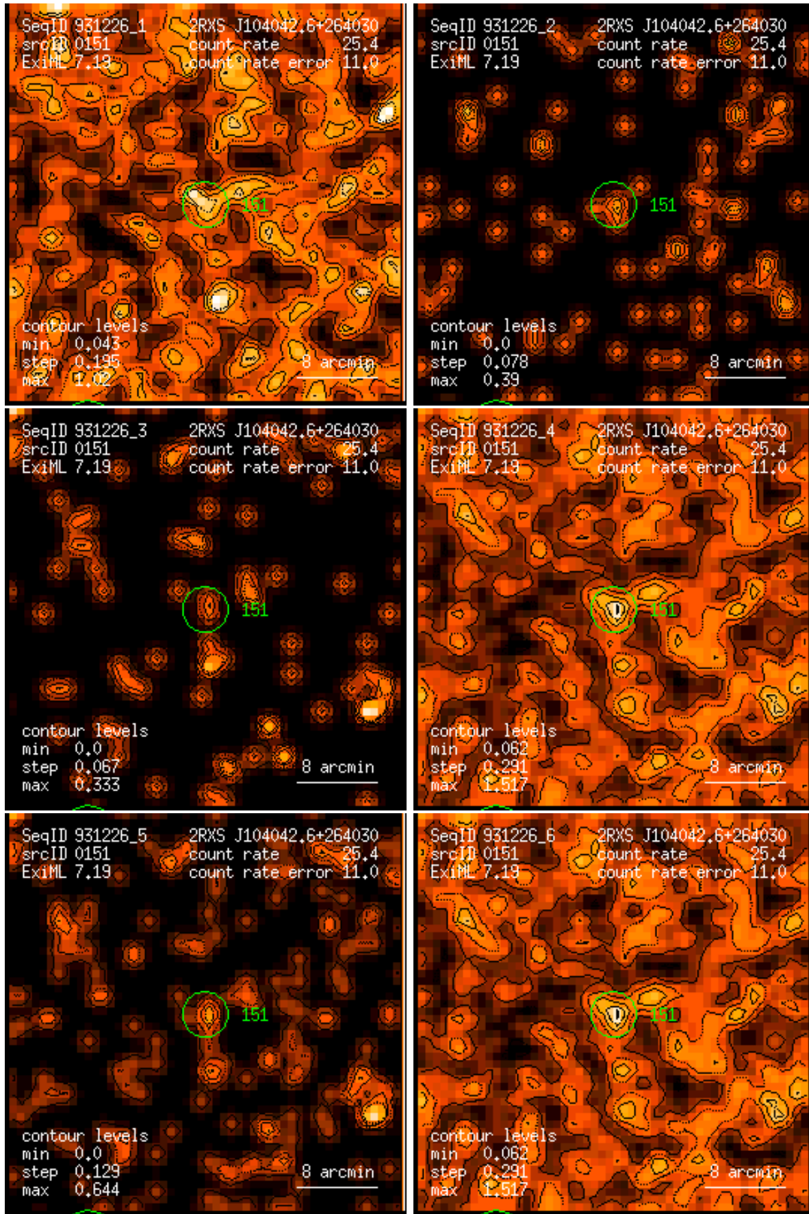
Figure 151: RASS 931226: detection 0151: band rate images, Gaussian filter: (1) PSPC channels 11 – 41, (2) 52 – 90, (3) 91 – 201, (4) 11 – 235, (5) 52 – 201, (6) 11 – 201. Broad band rates in counts/ks. Band rate contour levels in counts/ks/arcmin 2 .
