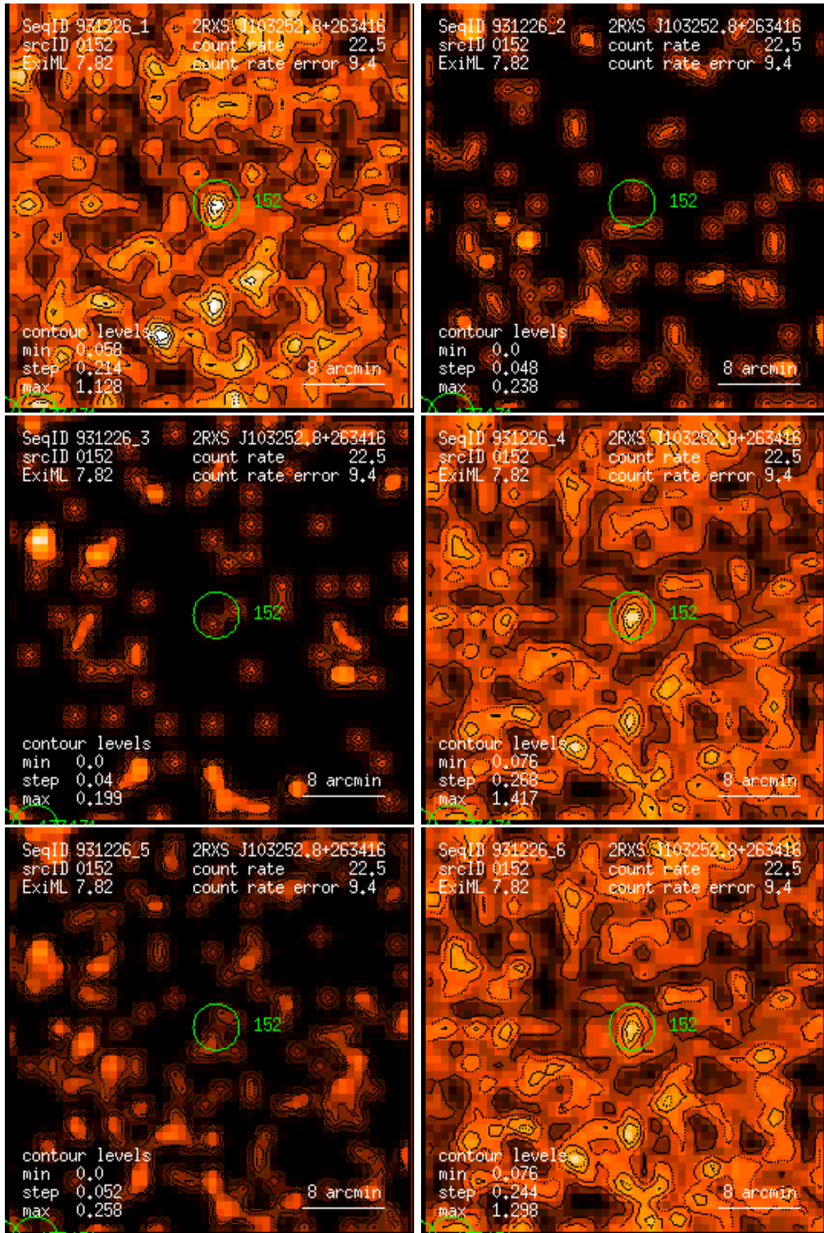
Figure 152: RASS 931226: detection 0152: band rate images, Gaussian filter: (1) PSPC channels 11 – 41, (2) 52 – 90, (3) 91 – 201, (4) 11 – 235, (5) 52 – 201, (6) 11 – 201. Broad band rates in counts/ks. Band rate contour levels in counts/ks/arcmin 2 .
