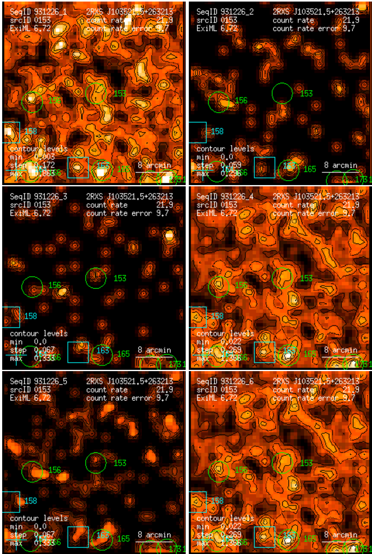
Figure 153: RASS 931226: detection 0153: band rate images, Gaussian filter: (1) PSPC channels 11 – 41, (2) 52 – 90, (3) 91 – 201, (4) 11 – 235, (5) 52 – 201, (6) 11 – 201. Broad band rates in counts/ks. Band rate contour levels in counts/ks/arcmin 2 .
