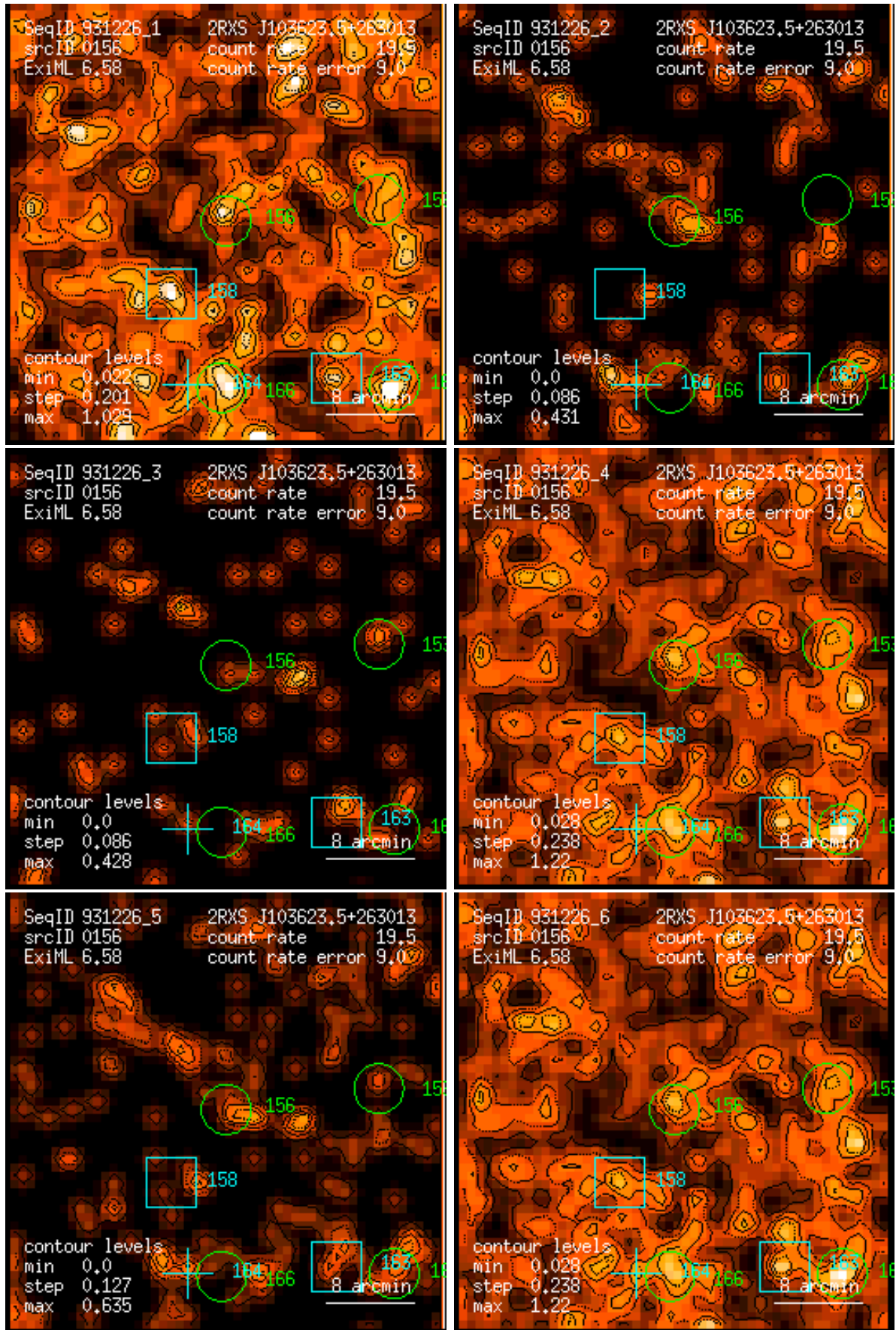
Figure 156: RASS 931226: detection 0156: band rate images, Gaussian filter: (1) PSPC channels 11 – 41, (2) 52 – 90, (3) 91 – 201, (4) 11 – 235, (5) 52 – 201, (6) 11 – 201. Broad band rates in counts/ks. Band rate contour levels in counts/ks/arcmin 2 .
