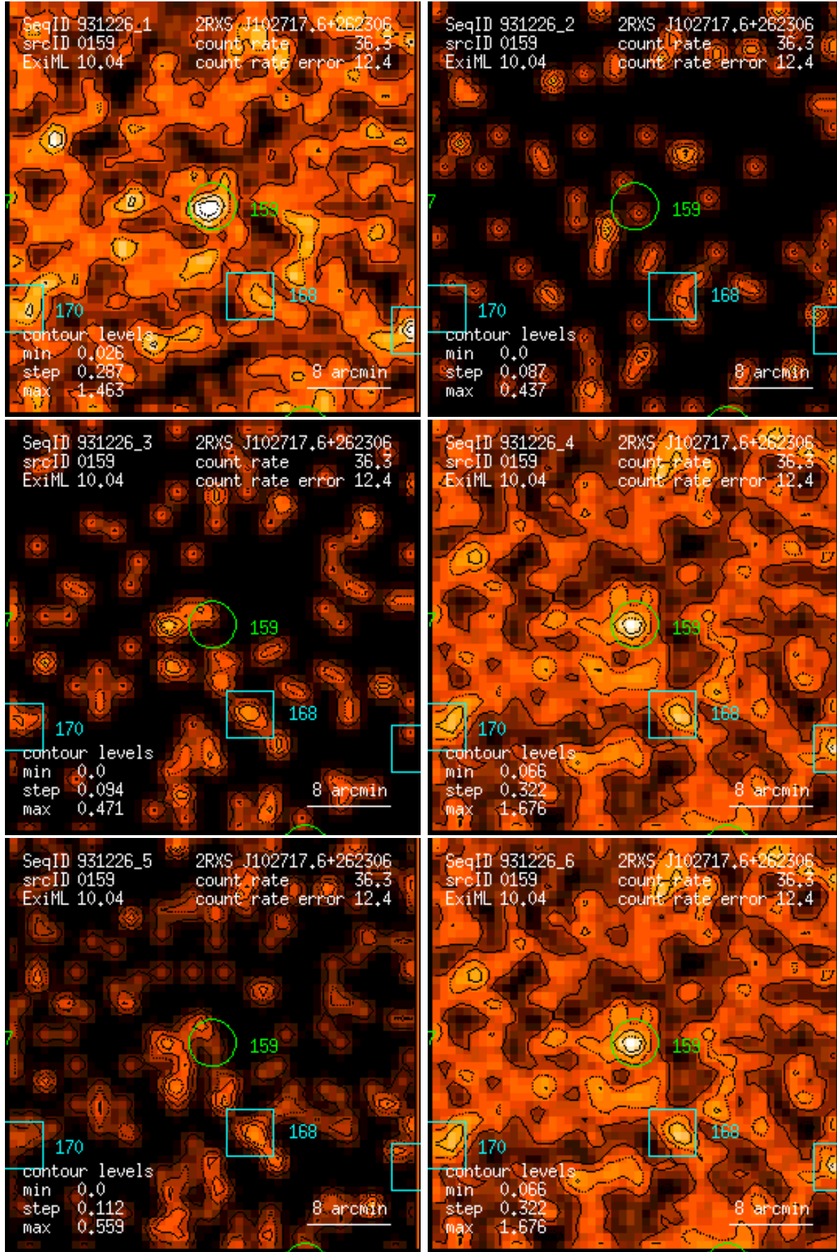
Figure 159: RASS 931226: detection 0159: band rate images, Gaussian filter: (1) PSPC channels 11 – 41, (2) 52 – 90, (3) 91 – 201, (4) 11 – 235, (5) 52 – 201, (6) 11 – 201. Broad band rates in counts/ks. Band rate contour levels in counts/ks/arcmin 2 .
