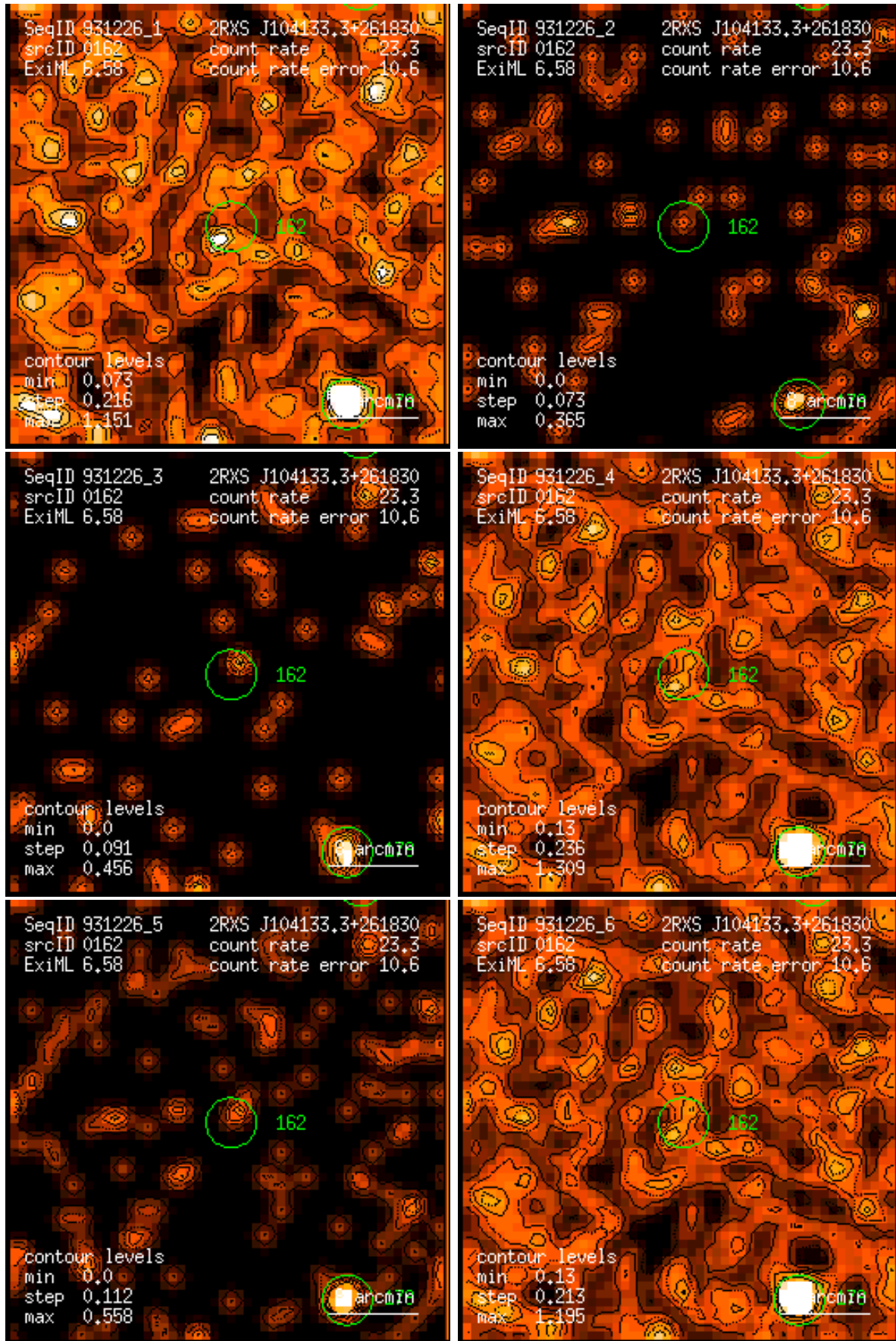
Figure 162: RASS 931226: detection 0162: band rate images, Gaussian filter: (1) PSPC channels 11 – 41, (2) 52 – 90, (3) 91 – 201, (4) 11 – 235, (5) 52 – 201, (6) 11 – 201. Broad band rates in counts/ks. Band rate contour levels in counts/ks/arcmin 2 .
