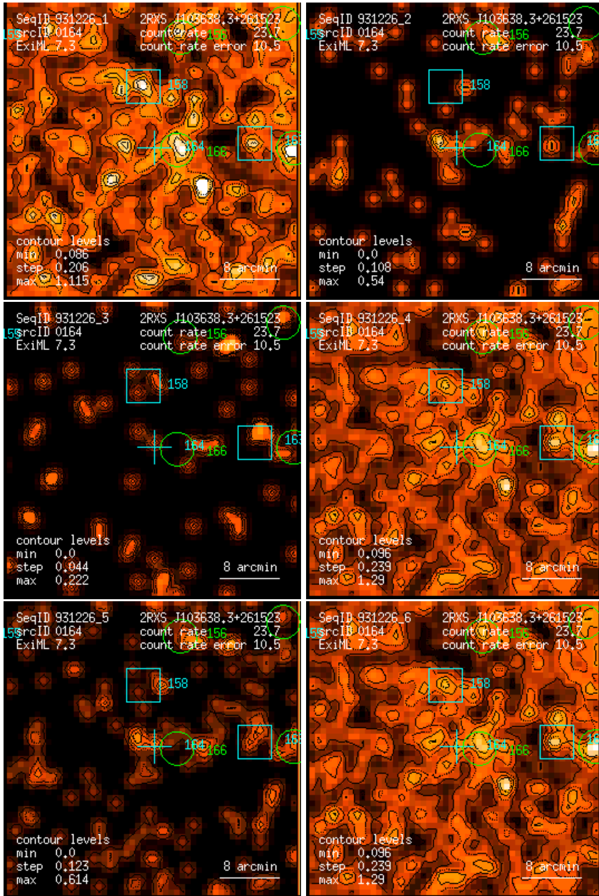
Figure 164: RASS 931226: detection 0164: band rate images, Gaussian filter: (1) PSPC channels 11 – 41, (2) 52 – 90, (3) 91 – 201, (4) 11 – 235, (5) 52 – 201, (6) 11 – 201. Broad band rates in counts/ks. Band rate contour levels in counts/ks/arcmin 2 .
