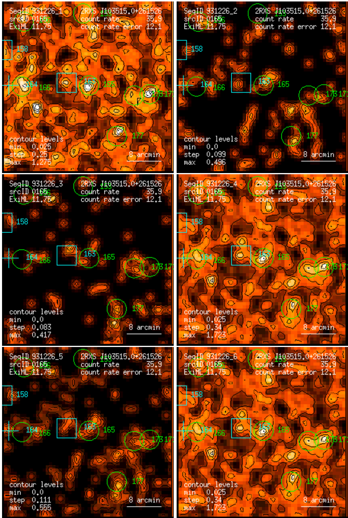
Figure 165: RASS 931226: detection 0165: band rate images, Gaussian filter: (1) PSPC channels 11 – 41, (2) 52 – 90, (3) 91 – 201, (4) 11 – 235, (5) 52 – 201, (6) 11 – 201. Broad band rates in counts/ks. Band rate contour levels in counts/ks/arcmin 2 .
