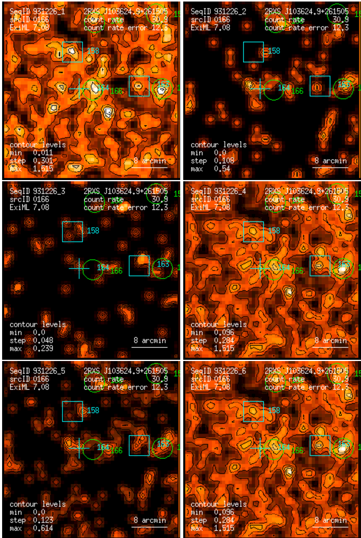
Figure 166: RASS 931226: detection 0166: band rate images, Gaussian filter: (1) PSPC channels 11 – 41, (2) 52 – 90, (3) 91 – 201, (4) 11 – 235, (5) 52 – 201, (6) 11 – 201. Broad band rates in counts/ks. Band rate contour levels in counts/ks/arcmin 2 .
