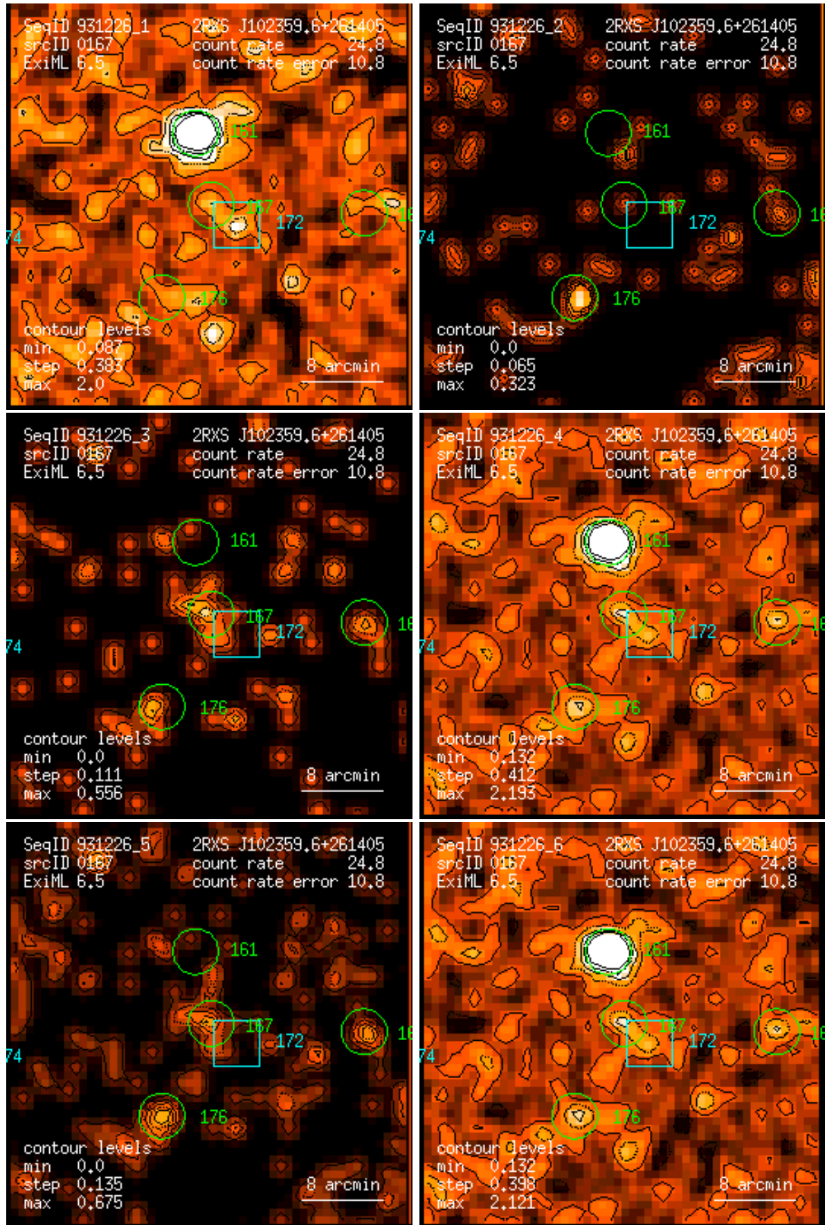
Figure 167: RASS 931226: detection 0167: band rate images, Gaussian filter: (1) PSPC channels 11 – 41, (2) 52 – 90, (3) 91 – 201, (4) 11 – 235, (5) 52 – 201, (6) 11 – 201. Broad band rates in counts/ks. Band rate contour levels in counts/ks/arcmin 2 .
