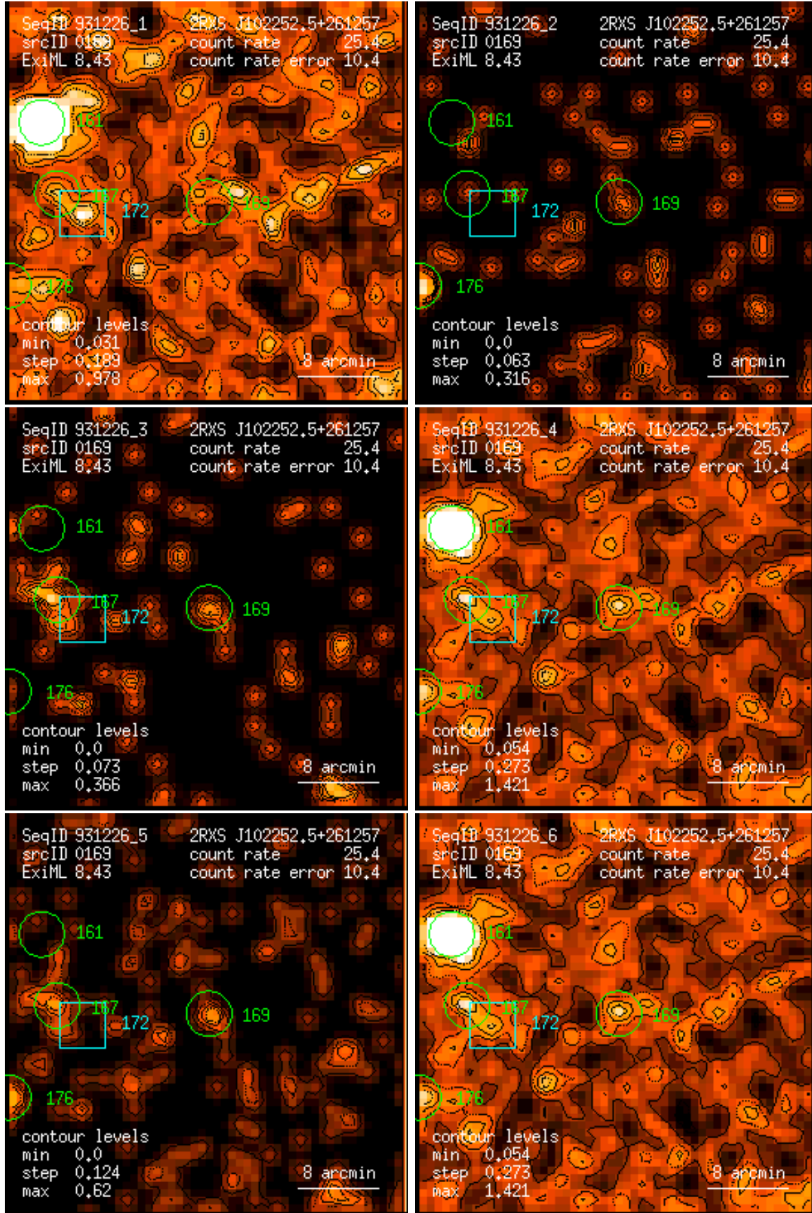
Figure 169: RASS 931226: detection 0169: band rate images, Gaussian filter: (1) PSPC channels 11 – 41, (2) 52 – 90, (3) 91 – 201, (4) 11 – 235, (5) 52 – 201, (6) 11 – 201. Broad band rates in counts/ks. Band rate contour levels in counts/ks/arcmin 2 .
