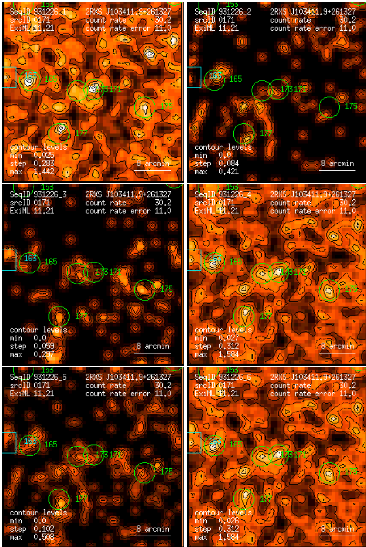
Figure 171: RASS 931226: detection 0171: band rate images, Gaussian filter: (1) PSPC channels 11 – 41, (2) 52 – 90, (3) 91 – 201, (4) 11 – 235, (5) 52 – 201, (6) 11 – 201. Broad band rates in counts/ks. Band rate contour levels in counts/ks/arcmin 2 .
