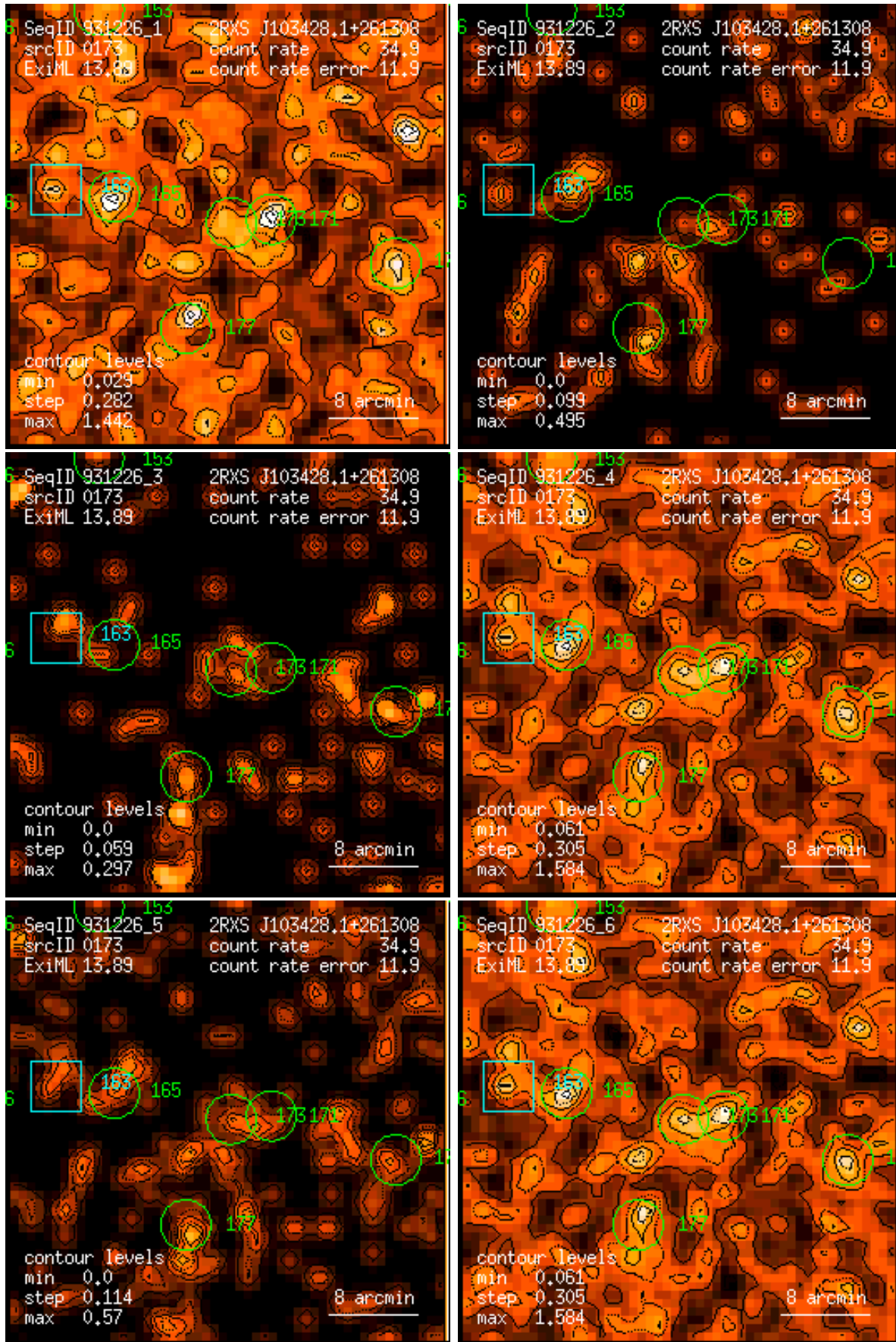
Figure 173: RASS 931226: detection 0173: band rate images, Gaussian filter: (1) PSPC channels 11 – 41, (2) 52 – 90, (3) 91 – 201, (4) 11 – 235, (5) 52 – 201, (6) 11 – 201. Broad band rates in counts/ks. Band rate contour levels in counts/ks/arcmin 2 .
