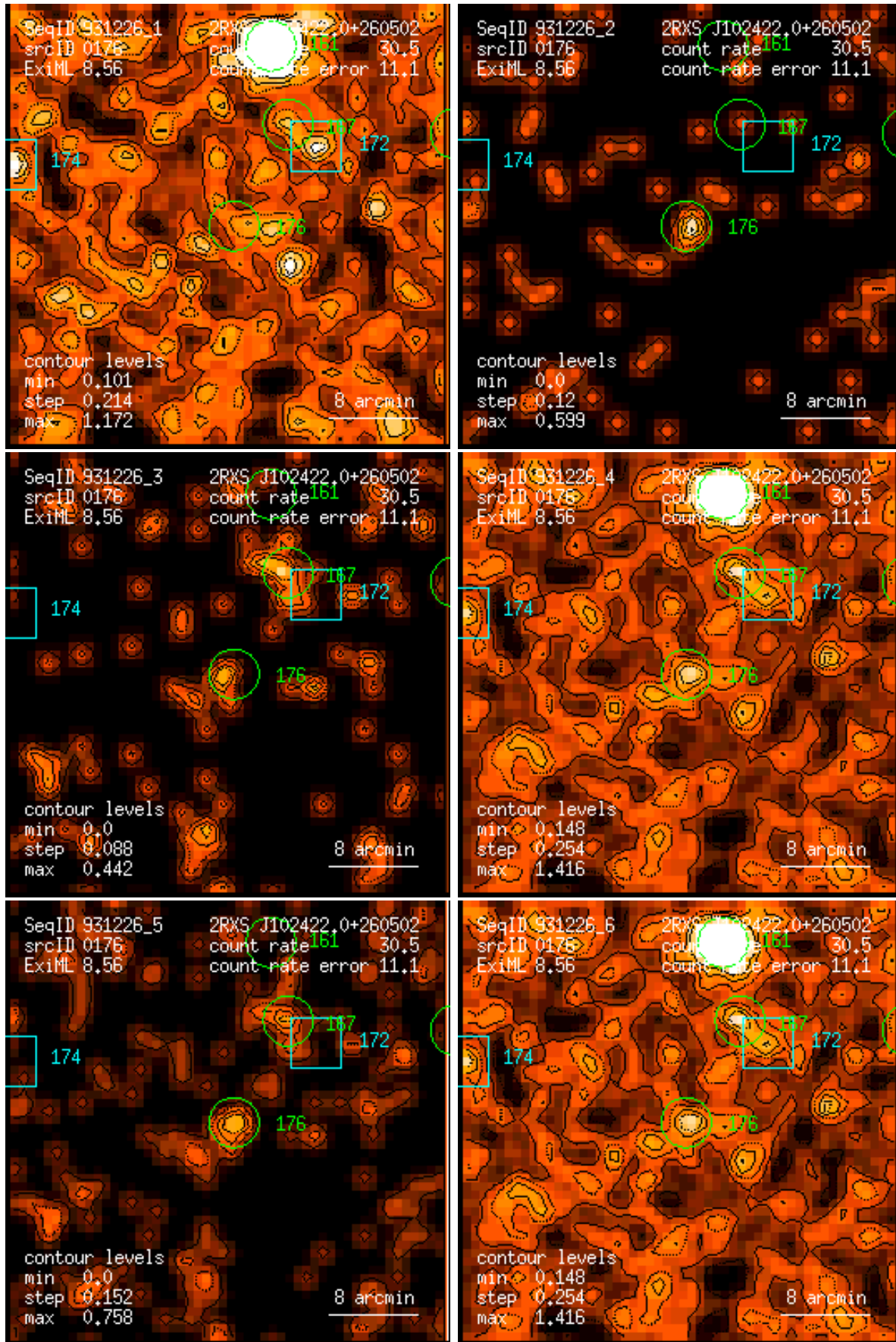
Figure 176: RASS 931226: detection 0176: band rate images, Gaussian filter: (1) PSPC channels 11 – 41, (2) 52 – 90, (3) 91 – 201, (4) 11 – 235, (5) 52 – 201, (6) 11 – 201. Broad band rates in counts/ks. Band rate contour levels in counts/ks/arcmin 2 .
