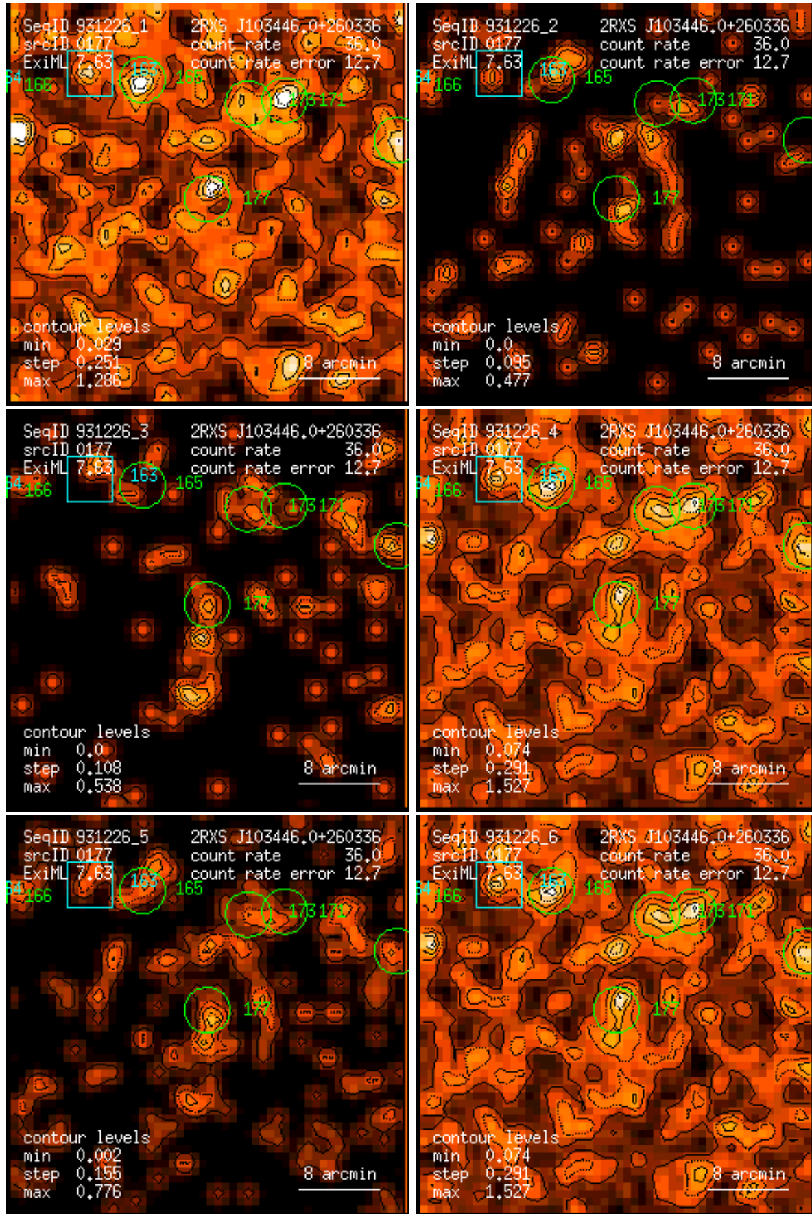
Figure 177: RASS 931226: detection 0177: band rate images, Gaussian filter: (1) PSPC channels 11 – 41, (2) 52 – 90, (3) 91 – 201, (4) 11 – 235, (5) 52 – 201, (6) 11 – 201. Broad band rates in counts/ks. Band rate contour levels in counts/ks/arcmin 2 .
