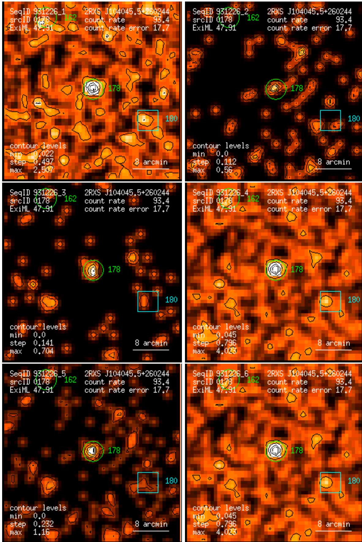
Figure 178: RASS 931226: detection 0178: band rate images, Gaussian filter: (1) PSPC channels 11 – 41, (2) 52 – 90, (3) 91 – 201, (4) 11 – 235, (5) 52 – 201, (6) 11 – 201. Broad band rates in counts/ks. Band rate contour levels in counts/ks/arcmin 2 .
