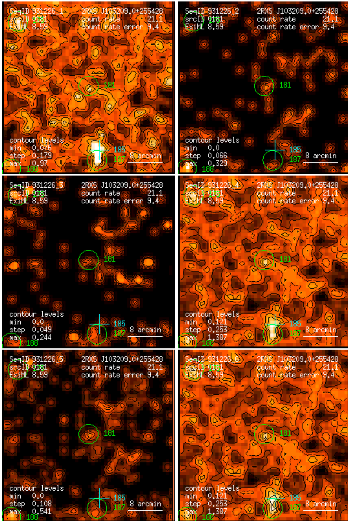
Figure 181: RASS 931226: detection 0181: band rate images, Gaussian filter: (1) PSPC channels 11 – 41, (2) 52 – 90, (3) 91 – 201, (4) 11 – 235, (5) 52 – 201, (6) 11 – 201. Broad band rates in counts/ks. Band rate contour levels in counts/ks/arcmin 2 .
