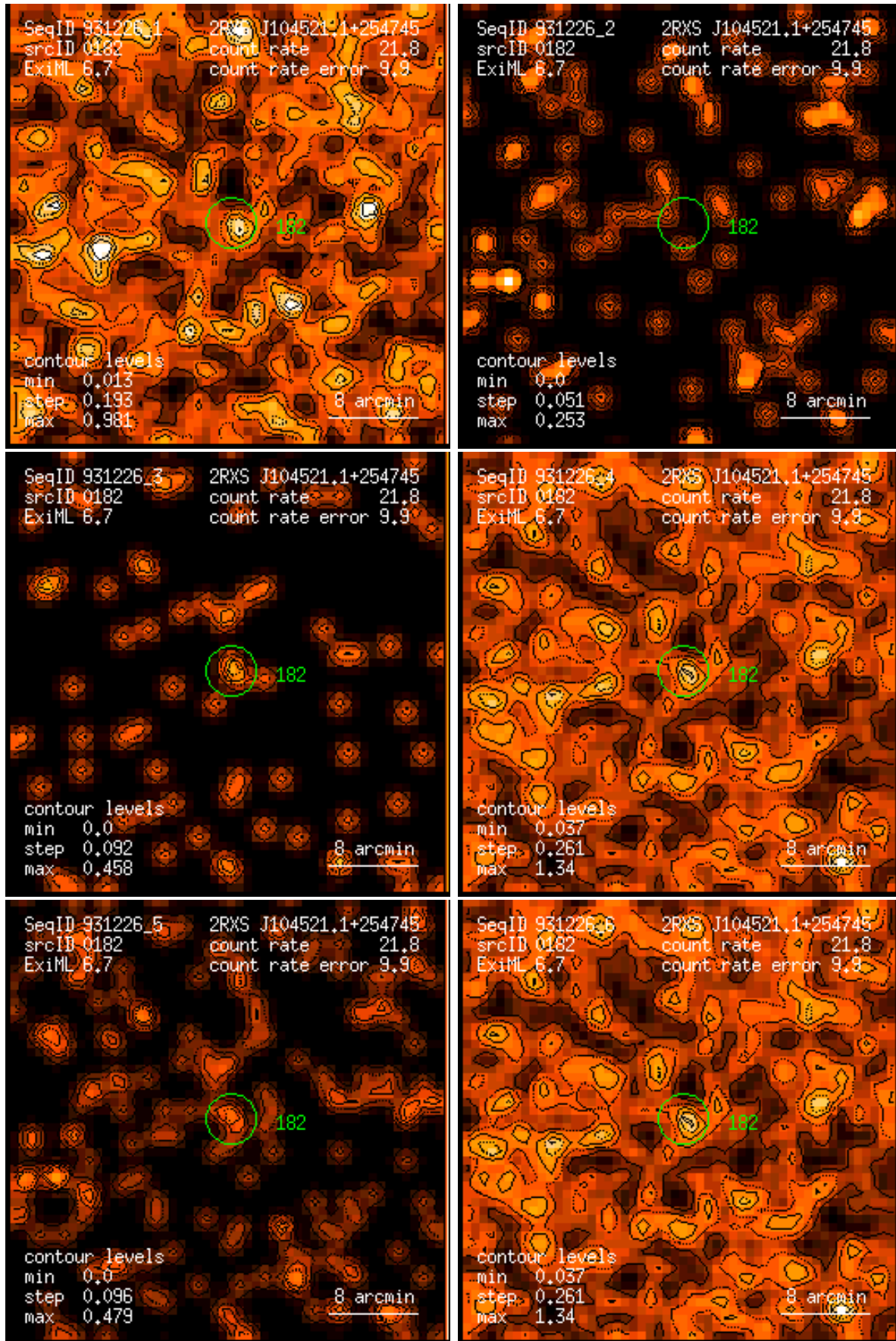
Figure 182: RASS 931226: detection 0182: band rate images, Gaussian filter: (1) PSPC channels 11 – 41, (2) 52 – 90, (3) 91 – 201, (4) 11 – 235, (5) 52 – 201, (6) 11 – 201. Broad band rates in counts/ks. Band rate contour levels in counts/ks/arcmin 2 .
