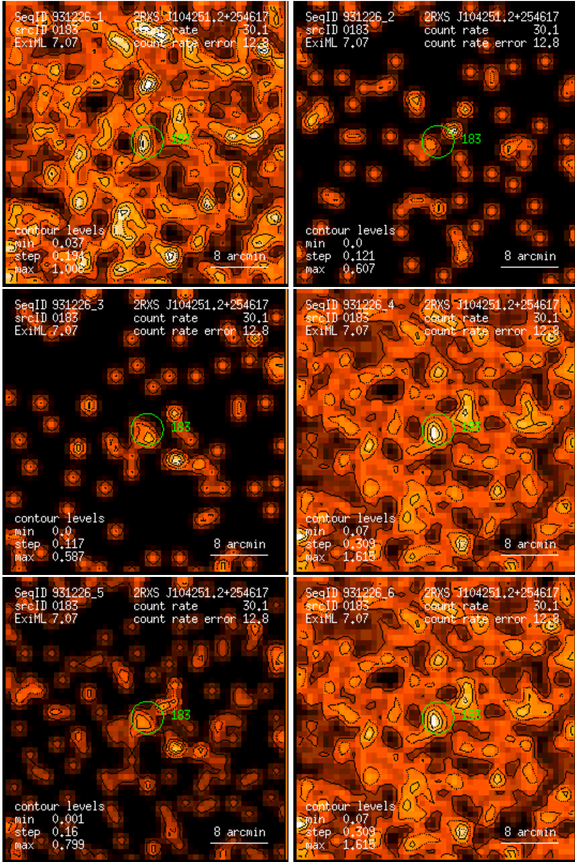
Figure 183: RASS 931226: detection 0183: band rate images, Gaussian filter: (1) PSPC channels 11 – 41, (2) 52 – 90, (3) 91 – 201, (4) 11 – 235, (5) 52 – 201, (6) 11 – 201. Broad band rates in counts/ks. Band rate contour levels in counts/ks/arcmin 2 .
