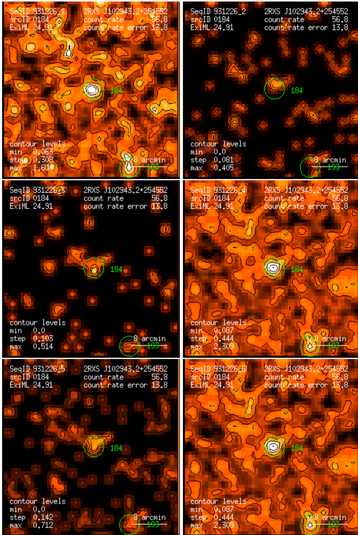
Figure 184: RASS 931226: detection 0184: band rate images, Gaussian filter: (1) PSPC channels 11 – 41, (2) 52 – 90, (3) 91 – 201, (4) 11 – 235, (5) 52 – 201, (6) 11 – 201. Broad band rates in counts/ks. Band rate contour levels in counts/ks/arcmin 2 .
