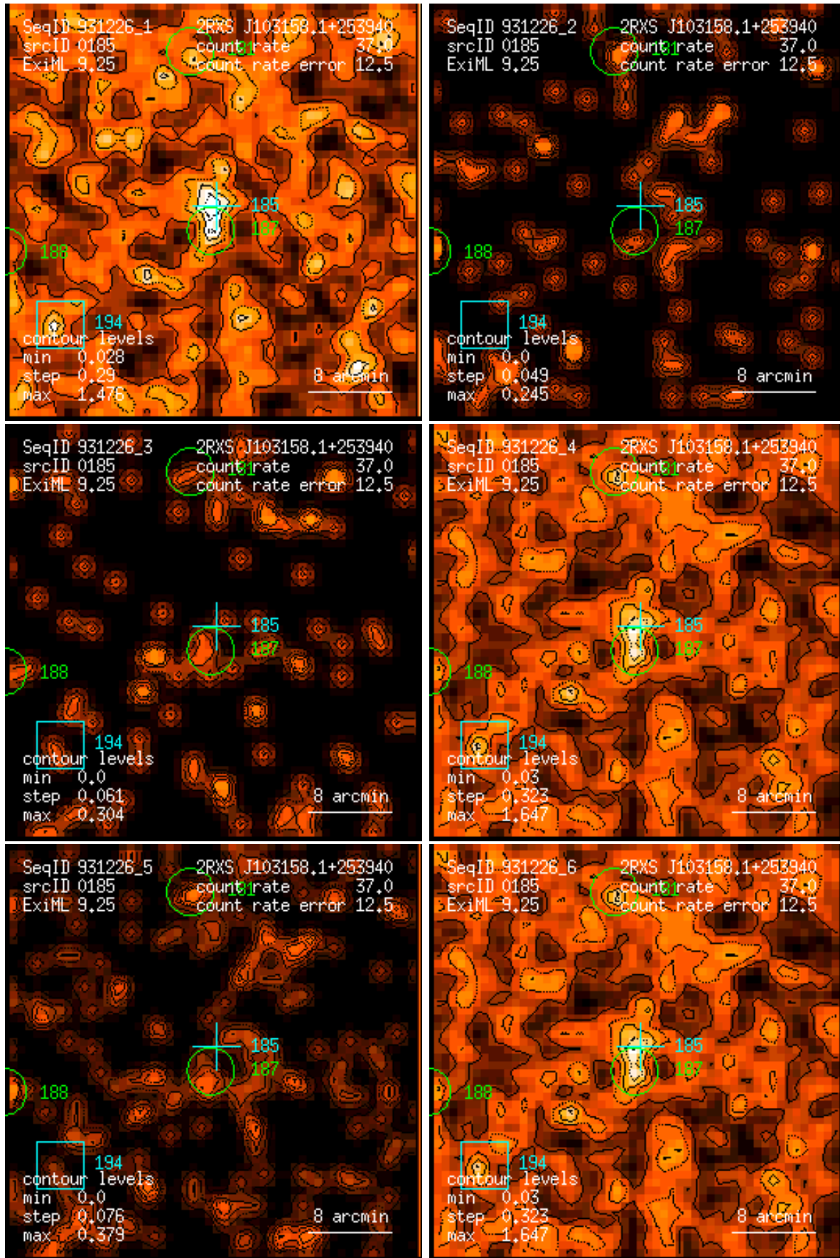
Figure 185: RASS 931226: detection 0185: band rate images, Gaussian filter: (1) PSPC channels 11 – 41, (2) 52 – 90, (3) 91 – 201, (4) 11 – 235, (5) 52 – 201, (6) 11 – 201. Broad band rates in counts/ks. Band rate contour levels in counts/ks/arcmin 2 .
