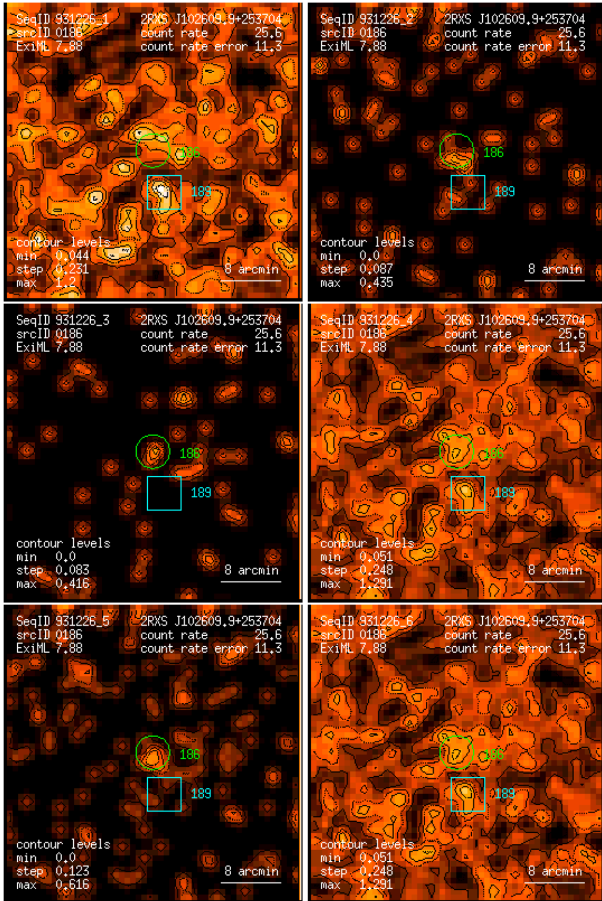
Figure 186: RASS 931226: detection 0186: band rate images, Gaussian filter: (1) PSPC channels 11 – 41, (2) 52 – 90, (3) 91 – 201, (4) 11 – 235, (5) 52 – 201, (6) 11 – 201. Broad band rates in counts/ks. Band rate contour levels in counts/ks/arcmin 2 .
