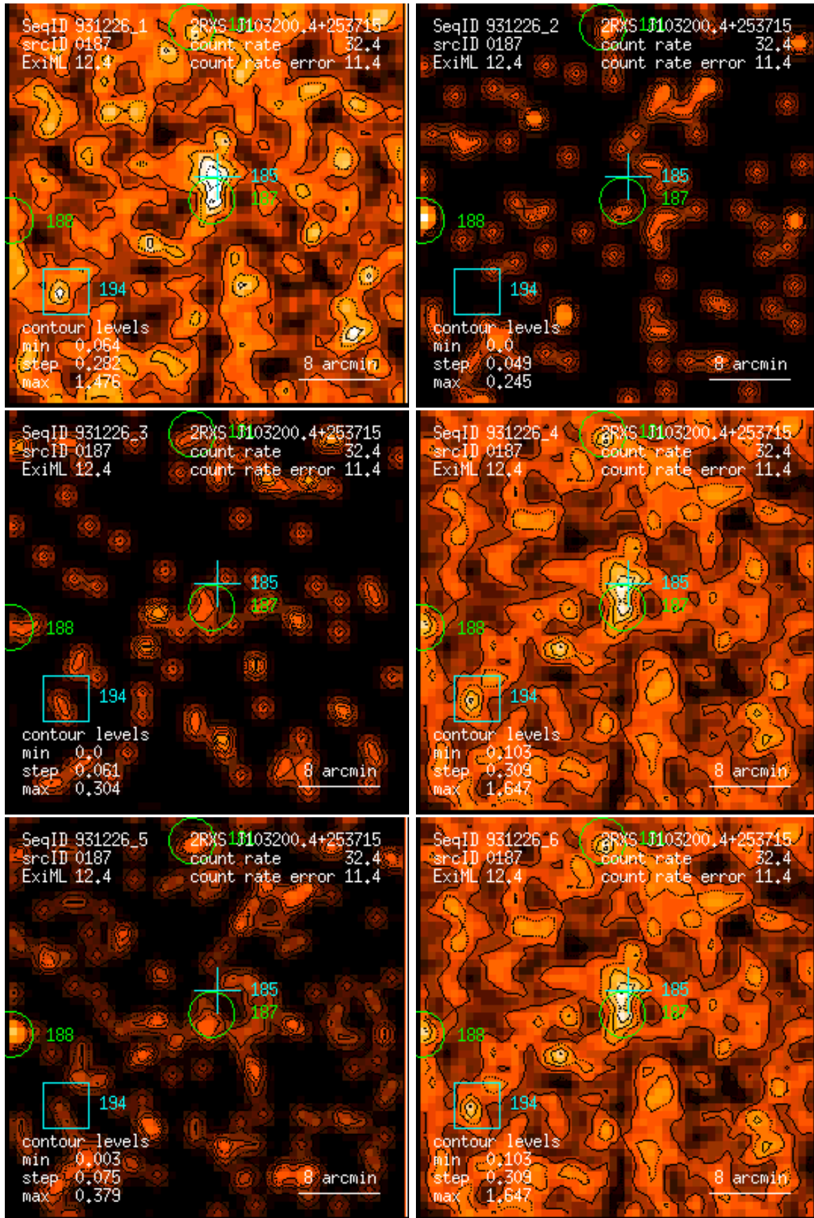
Figure 187: RASS 931226: detection 0187: band rate images, Gaussian filter: (1) PSPC channels 11 – 41, (2) 52 – 90, (3) 91 – 201, (4) 11 – 235, (5) 52 – 201, (6) 11 – 201. Broad band rates in counts/ks. Band rate contour levels in counts/ks/arcmin 2 .
