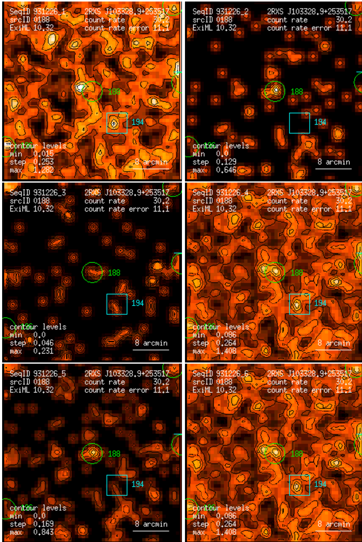
Figure 188: RASS 931226: detection 0188: band rate images, Gaussian filter: (1) PSPC channels 11 – 41, (2) 52 – 90, (3) 91 – 201, (4) 11 – 235, (5) 52 – 201, (6) 11 – 201. Broad band rates in counts/ks. Band rate contour levels in counts/ks/arcmin 2 .
