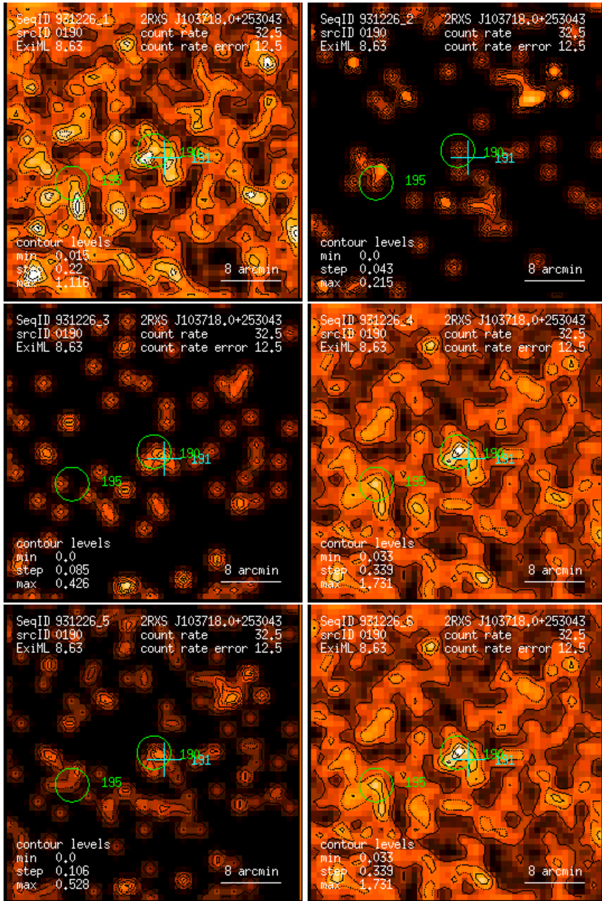
Figure 190: RASS 931226: detection 0190: band rate images, Gaussian filter: (1) PSPC channels 11 – 41, (2) 52 – 90, (3) 91 – 201, (4) 11 – 235, (5) 52 – 201, (6) 11 – 201. Broad band rates in counts/ks. Band rate contour levels in counts/ks/arcmin 2 .
