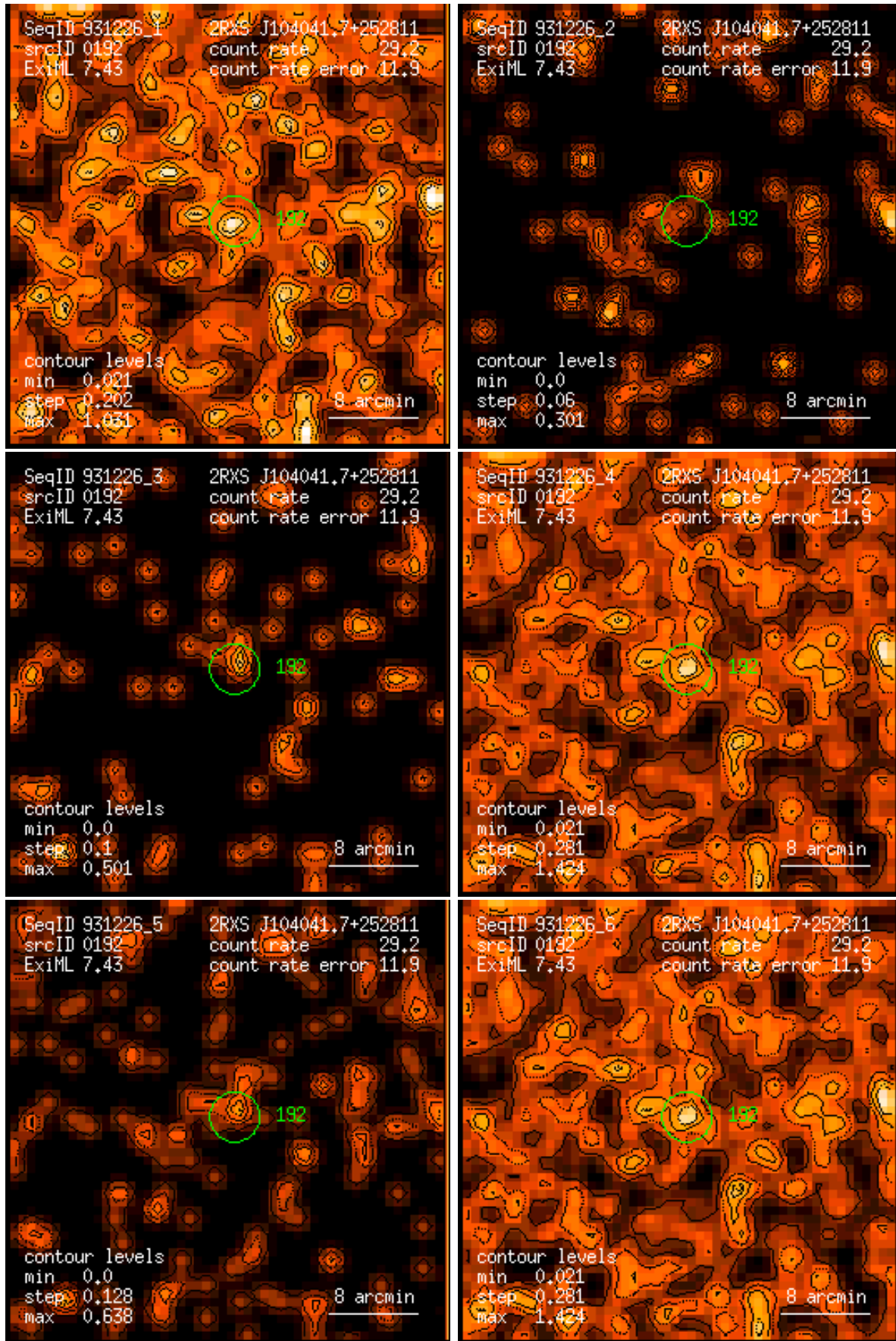
Figure 192: RASS 931226: detection 0192: band rate images, Gaussian filter: (1) PSPC channels 11 – 41, (2) 52 – 90, (3) 91 – 201, (4) 11 – 235, (5) 52 – 201, (6) 11 – 201. Broad band rates in counts/ks. Band rate contour levels in counts/ks/arcmin 2 .
