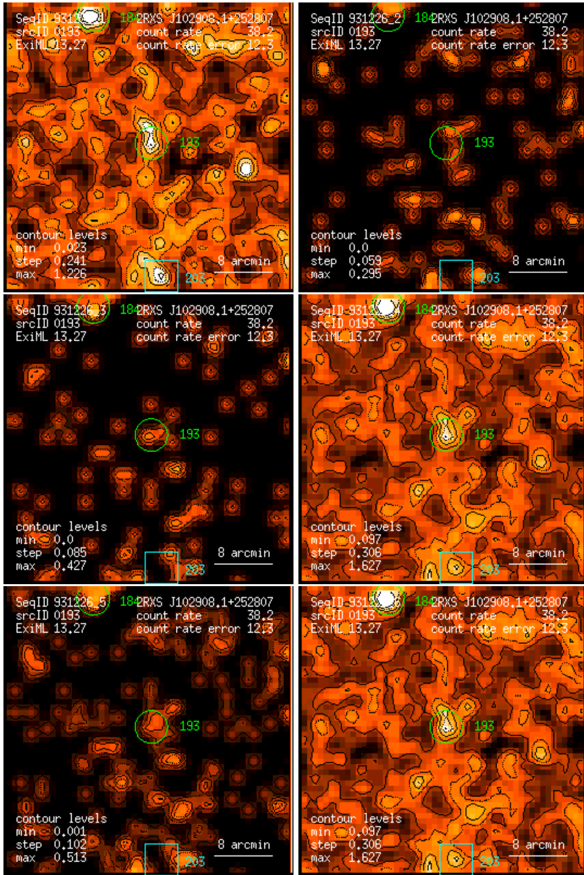
Figure 193: RASS 931226: detection 0193: band rate images, Gaussian filter: (1) PSPC channels 11 – 41, (2) 52 – 90, (3) 91 – 201, (4) 11 – 235, (5) 52 – 201, (6) 11 – 201. Broad band rates in counts/ks. Band rate contour levels in counts/ks/arcmin 2 .
