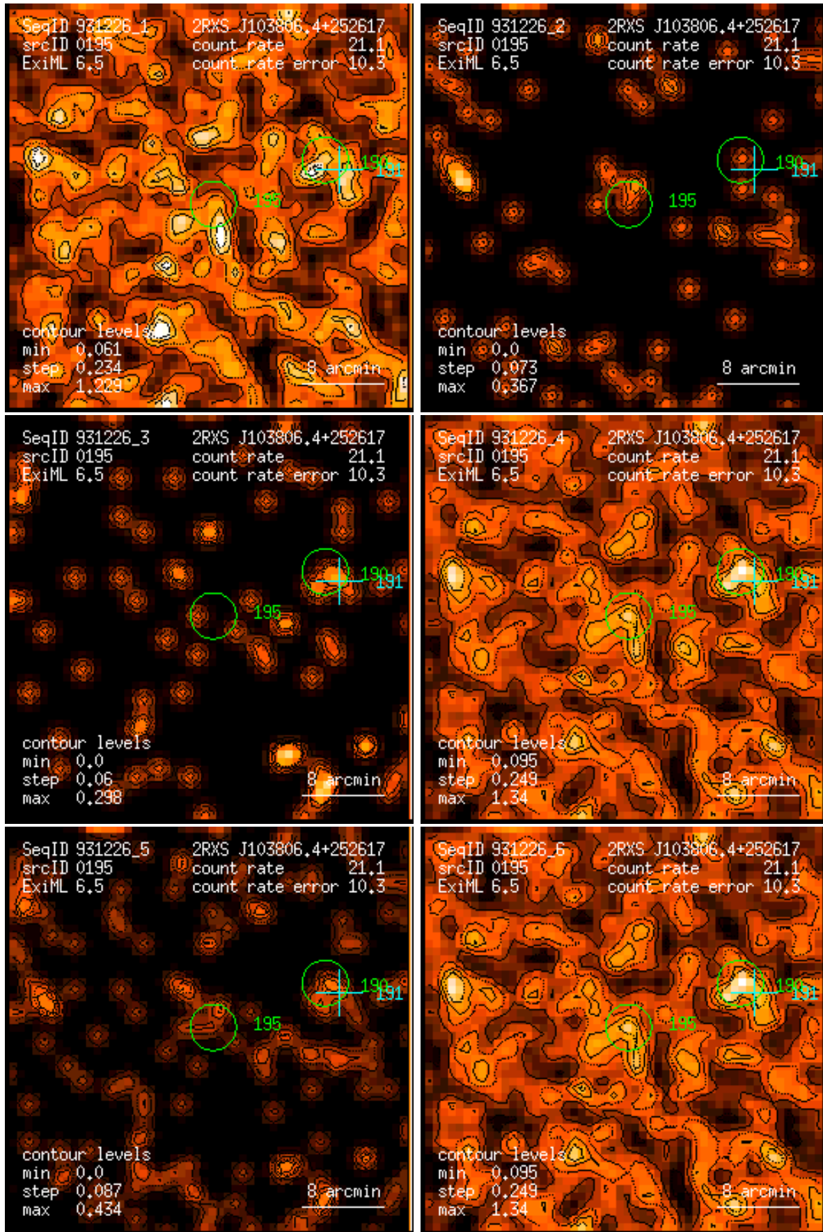
Figure 195: RASS 931226: detection 0195: band rate images, Gaussian filter: (1) PSPC channels 11 – 41, (2) 52 – 90, (3) 91 – 201, (4) 11 – 235, (5) 52 – 201, (6) 11 – 201. Broad band rates in counts/ks. Band rate contour levels in counts/ks/arcmin 2 .
