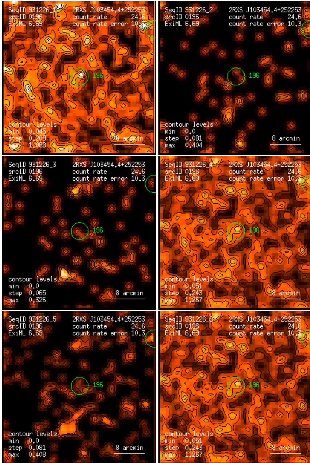
Figure 196: RASS 931226: detection 0196: band rate images, Gaussian filter: (1) PSPC channels 11 – 41, (2) 52 – 90, (3) 91 – 201, (4) 11 – 235, (5) 52 – 201, (6) 11 – 201. Broad band rates in counts/ks. Band rate contour levels in counts/ks/arcmin 2 .
