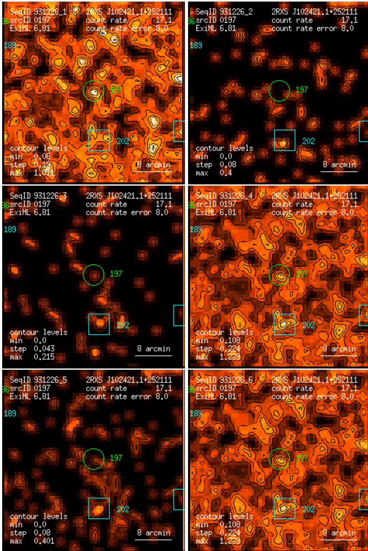
Figure 197: RASS 931226: detection 0197: band rate images, Gaussian filter: (1) PSPC channels 11 – 41, (2) 52 – 90, (3) 91 – 201, (4) 11 – 235, (5) 52 – 201, (6) 11 – 201. Broad band rates in counts/ks. Band rate contour levels in counts/ks/arcmin 2 .
