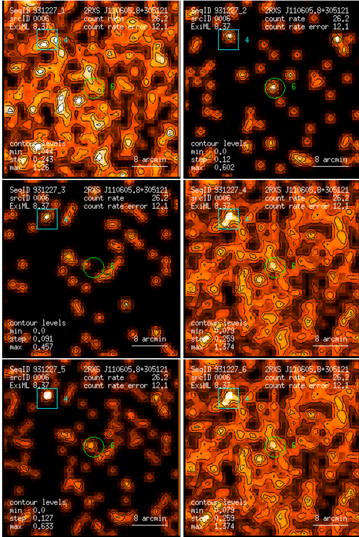
Figure 6: RASS 931227: detection 0006: band rate images, Gaussian filter: (1) PSPC channels 11 – 41, (2) 52 – 90, (3) 91 – 201, (4) 11 – 235, (5) 52 – 201, (6) 11 – 201. Broad band rates in counts/ks. Band rate contour levels in counts/ks/arcmin 2 .
