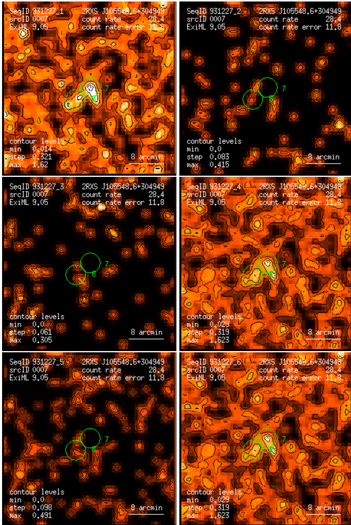
Figure 7: RASS 931227: detection 0007: band rate images, Gaussian filter: (1) PSPC channels 11 – 41, (2) 52 – 90, (3) 91 – 201, (4) 11 – 235, (5) 52 – 201, (6) 11 – 201. Broad band rates in counts/ks. Band rate contour levels in counts/ks/arcmin 2 .
