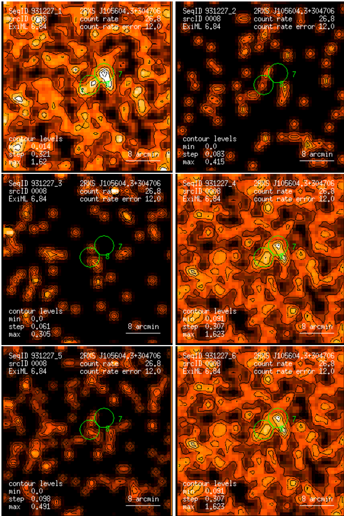
Figure 8: RASS 931227: detection 0008: band rate images, Gaussian filter: (1) PSPC channels 11 – 41, (2) 52 – 90, (3) 91 – 201, (4) 11 – 235, (5) 52 – 201, (6) 11 – 201. Broad band rates in counts/ks. Band rate contour levels in counts/ks/arcmin 2 .
