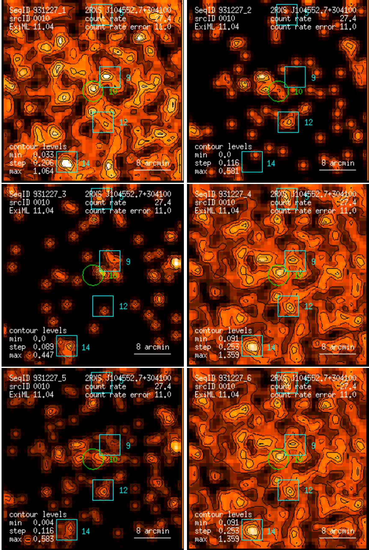
Figure 10: RASS 931227: detection 0010: band rate images, Gaussian filter: (1) PSPC channels 11 – 41, (2) 52 – 90, (3) 91 – 201, (4) 11 – 235, (5) 52 – 201, (6) 11 – 201. Broad band rates in counts/ks. Band rate contour levels in counts/ks/arcmin 2 .
