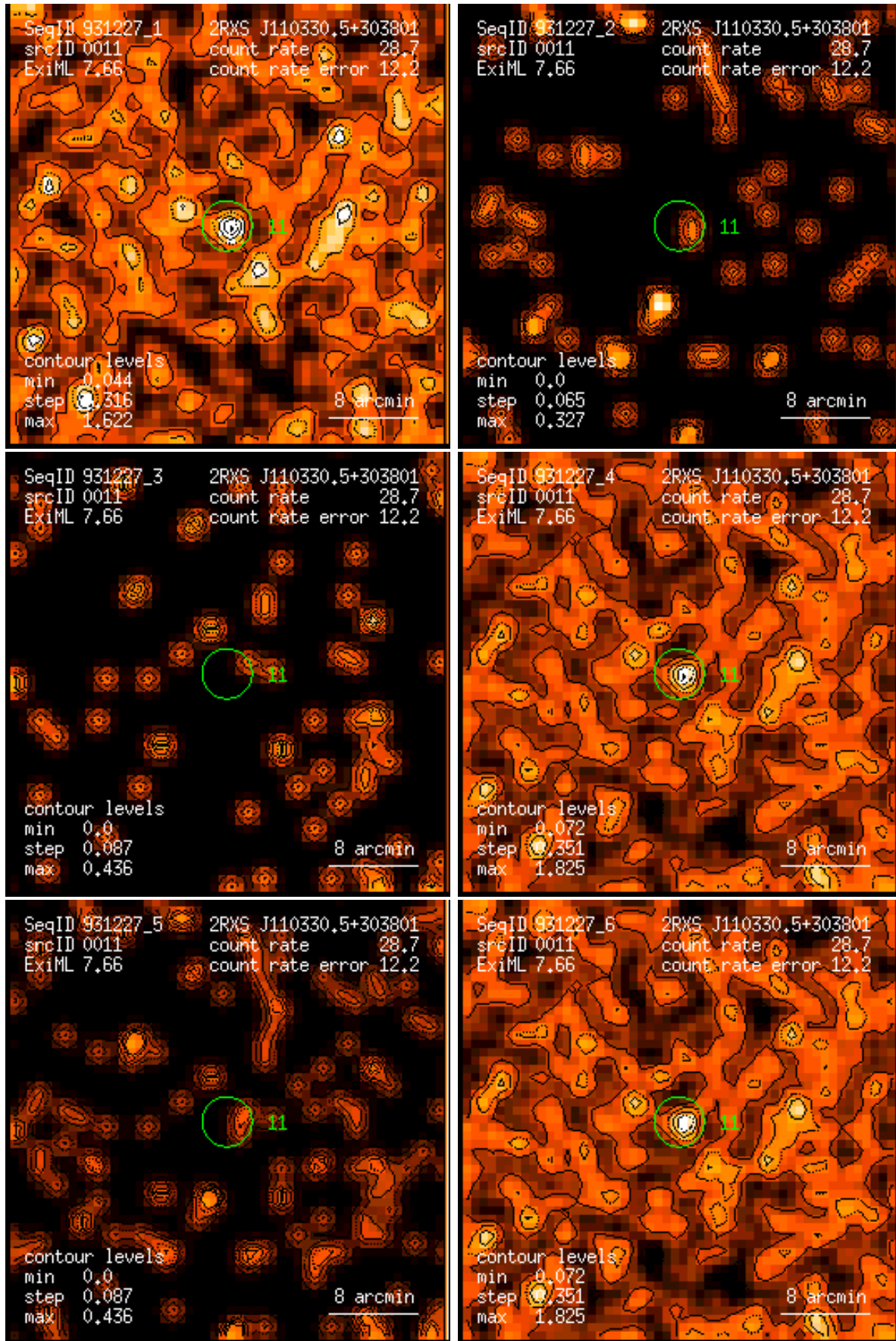
Figure 11: RASS 931227: detection 0011: band rate images, Gaussian filter: (1) PSPC channels 11 – 41, (2) 52 – 90, (3) 91 – 201, (4) 11 – 235, (5) 52 – 201, (6) 11 – 201. Broad band rates in counts/ks. Band rate contour levels in counts/ks/arcmin 2 .
