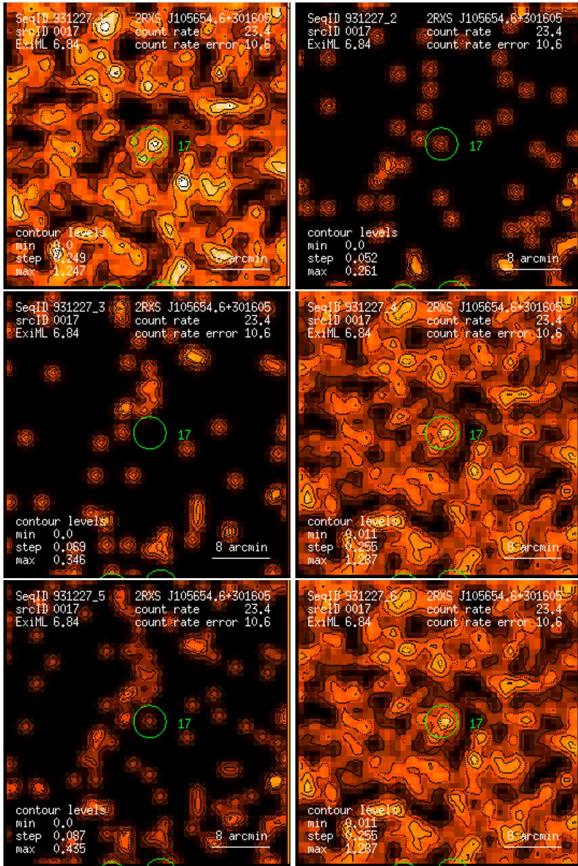
Figure 17: RASS 931227: detection 0017: band rate images, Gaussian filter: (1) PSPC channels 11 – 41, (2) 52 – 90, (3) 91 – 201, (4) 11 – 235, (5) 52 – 201, (6) 11 – 201. Broad band rates in counts/ks. Band rate contour levels in counts/ks/arcmin 2 .
