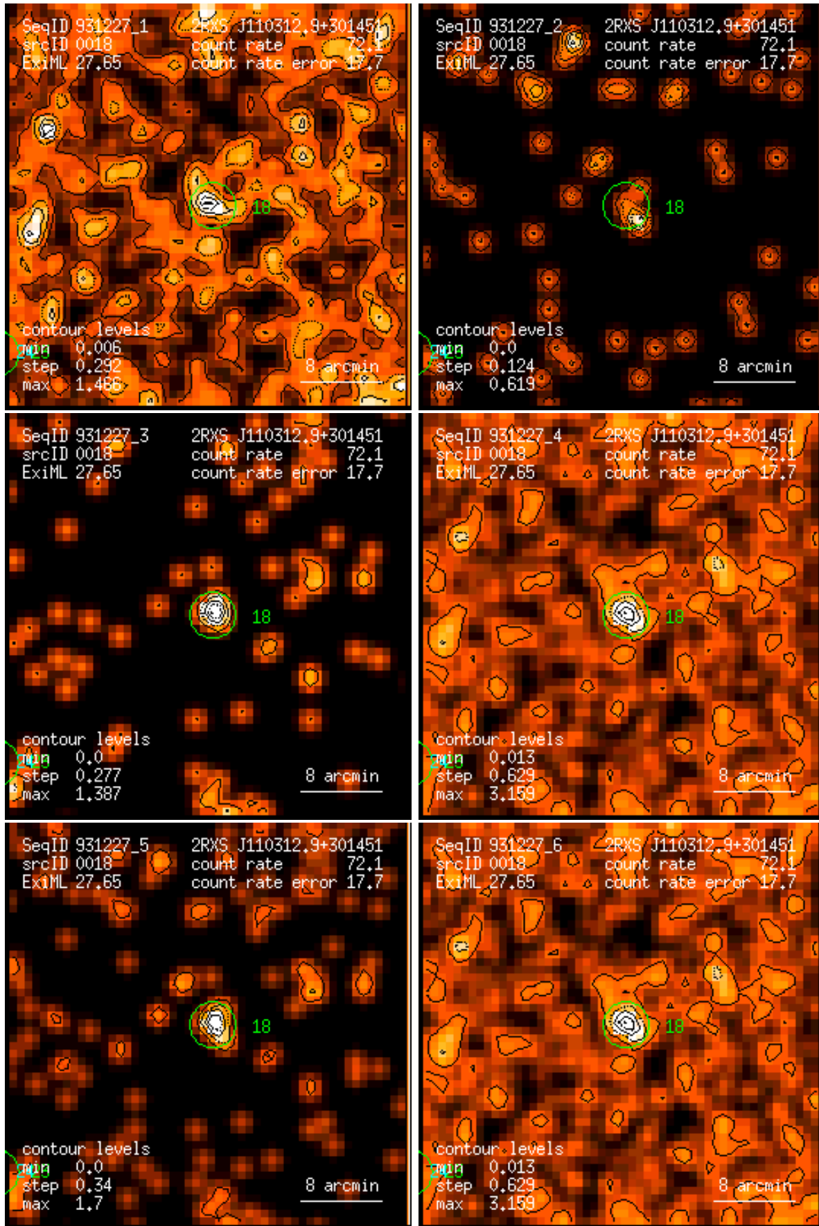
Figure 18: RASS 931227: detection 0018: band rate images, Gaussian filter: (1) PSPC channels 11 – 41, (2) 52 – 90, (3) 91 – 201, (4) 11 – 235, (5) 52 – 201, (6) 11 – 201. Broad band rates in counts/ks. Band rate contour levels in counts/ks/arcmin 2 .
