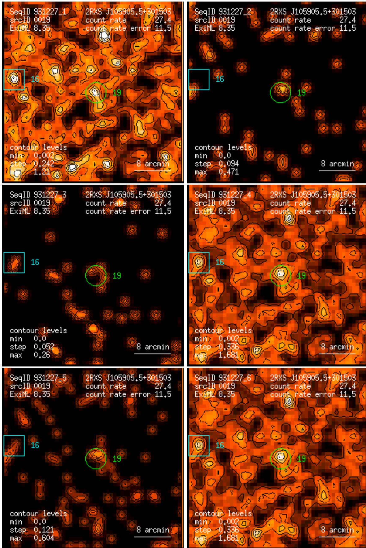
Figure 19: RASS 931227: detection 0019: band rate images, Gaussian filter: (1) PSPC channels 11 – 41, (2) 52 – 90, (3) 91 – 201, (4) 11 – 235, (5) 52 – 201, (6) 11 – 201. Broad band rates in counts/ks. Band rate contour levels in counts/ks/arcmin 2 .
